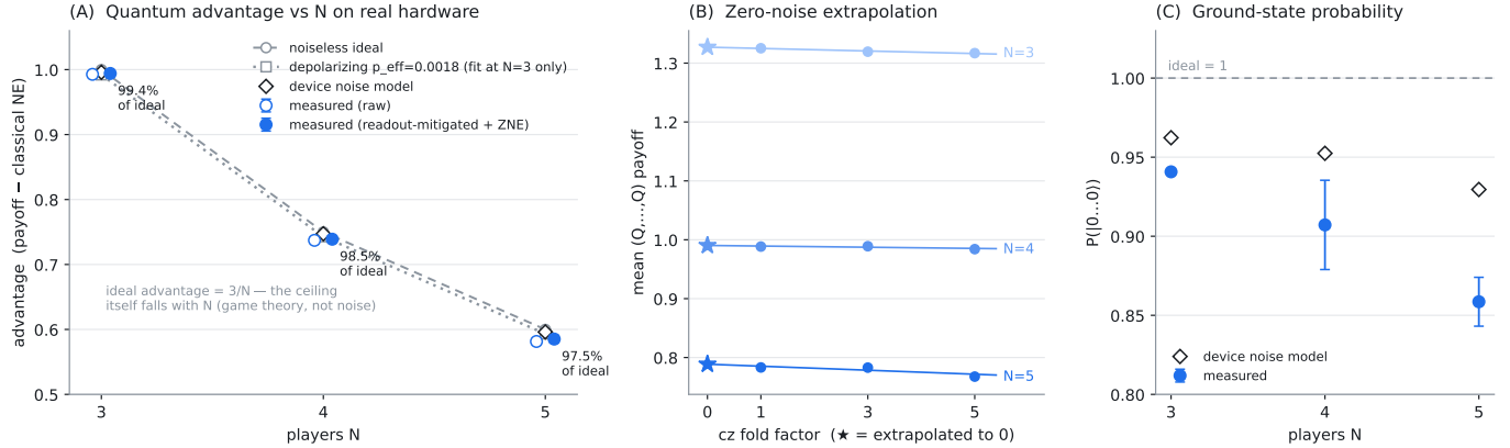
Fig. 7. Cross-calibration aggregate of the N -player GHZ EWL quantum advantage on ibm_fez (IBM Heron r2): three executions spanning two distinct provider calibrations , all on the same physical chain [59, 75, 74, 73, 79], 4096 shots each. Executions sharing a calibration stamp are averaged into one point before the spread is taken, because two runs under one calibration are one sample rather than two; the two epochs are 2026-07-16 08:30:13 (two executions) and 2026-07-26 13:29:01 (one). A fourth execution exists on chain [20, 21, 22, 23, 24] and is deliberately excluded here: pooling it would confound calibration drift with a change of physical qubits. Table III reports the registration-source execution alone. (A) Measured cooperative-profile advantage (mean (Q, \dots, Q) payoff minus the analytic noiseless classical-Nash payoff) at N = 3, 4, 5 : raw (open) and readout-mitigated + ZNE (filled), against the noiseless ideal (1.0, 0.75, 0.6), the device noise-model prediction (diamonds), and a single-parameter depolarizing model with p_{\text{eff}} = 0.0018 fitted to the N=3 point alone; its N=4, 5 values are predictions, not fits. The ideal, device-model and depolarizing curves are the registration anchor’s rather than run averages, so the registered p_{\text{eff}} is quoted unchanged. Error bars are the sample standard deviation across the two calibration epochs, a genuine cross-calibration estimate unlike the within-epoch spread reported in earlier drafts, and still exclude the within-run multinomial and weighted-fit standard errors, so they are a lower bound on total uncertainty. (B) ZNE mechanics: readout-mitigated payoff vs cz fold factor ( \lambda = 1, 3, 5 ) with the weighted linear fit extrapolated to \lambda = 0 (stars). (C) Ground-state probability P(|0 \dots 0\rangle) : the all-zero target-state population decays several times faster than the advantage because the mean-payoff observable is first-order insensitive to single bit-flips from |0 \dots 0\rangle . (Q, \dots, Q) passes the restricted-menu pure-Nash check only at N=3 among the plotted genuinely multiplayer cases; at N=4, 5 the profile is the cooperative quantum protocol, not an equilibrium.
