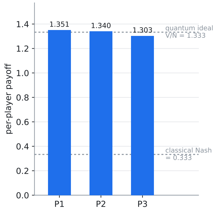
(B) Per-player payoff & quantum advantage
