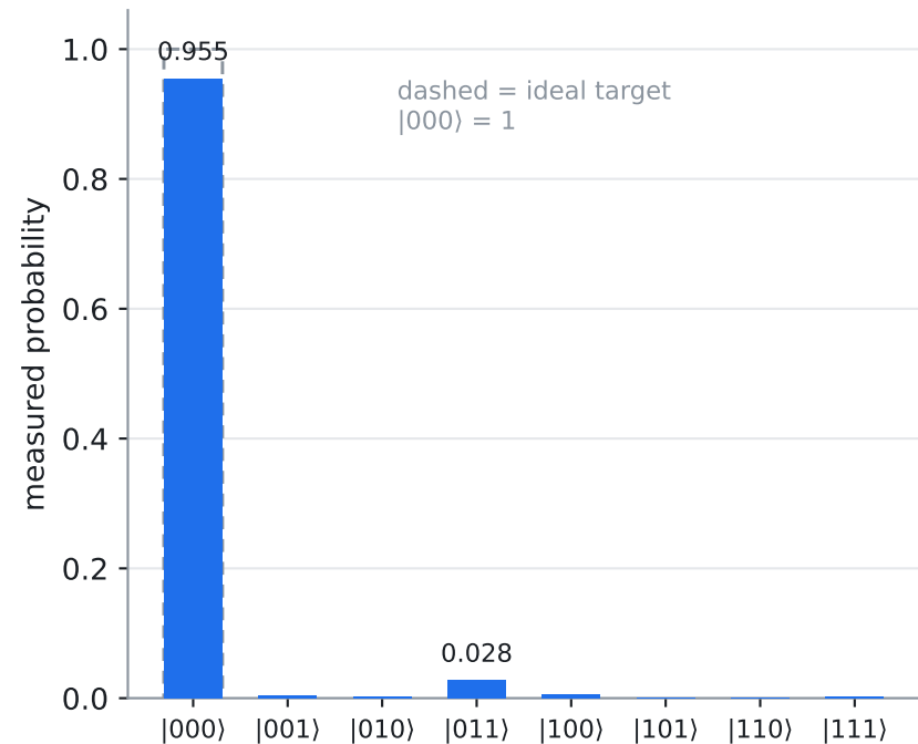
(A) Measured (Q,Q,Q) output distribution
