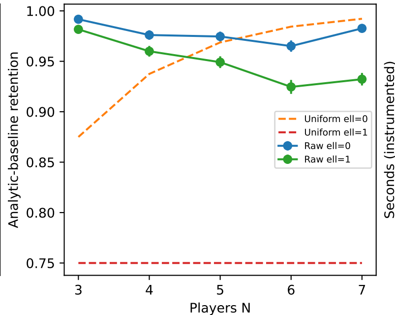
Payoff sensitivity
