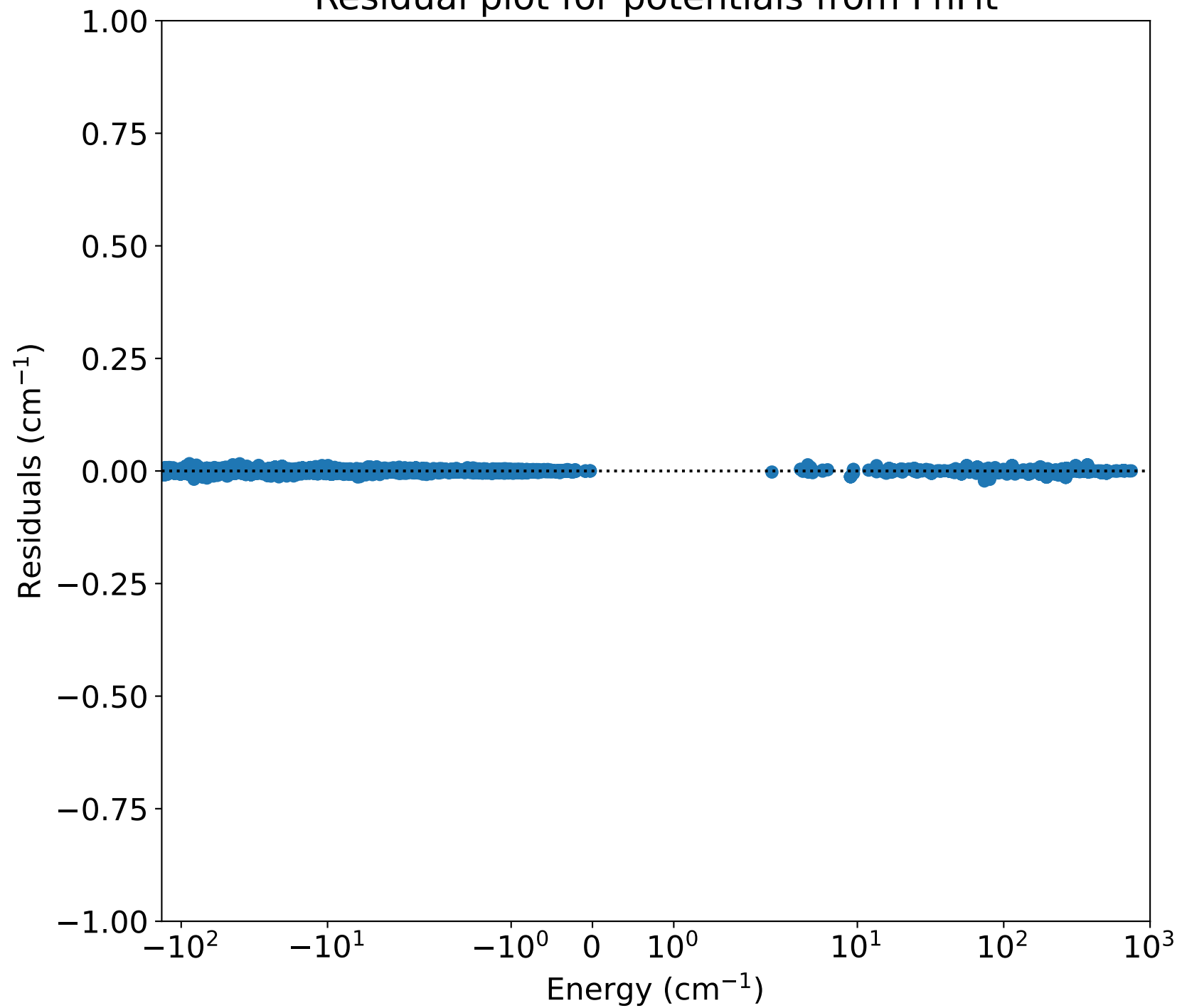
Residual plot for potentials from FnFit
