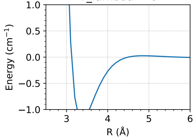
V_{\text{lambda}} = 6
