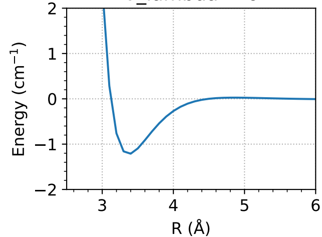
V_{\text{lambda}} = 6
