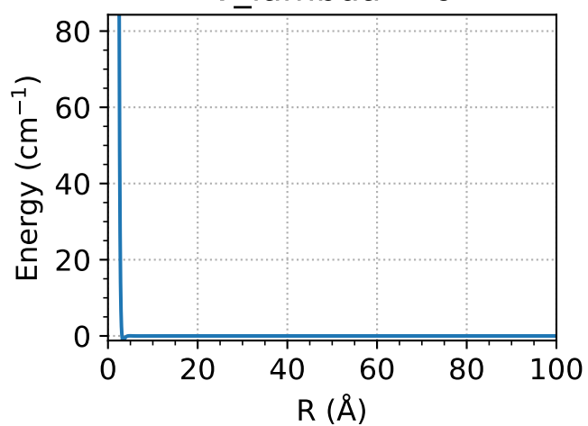
V_{\text{lambda}} = 6
