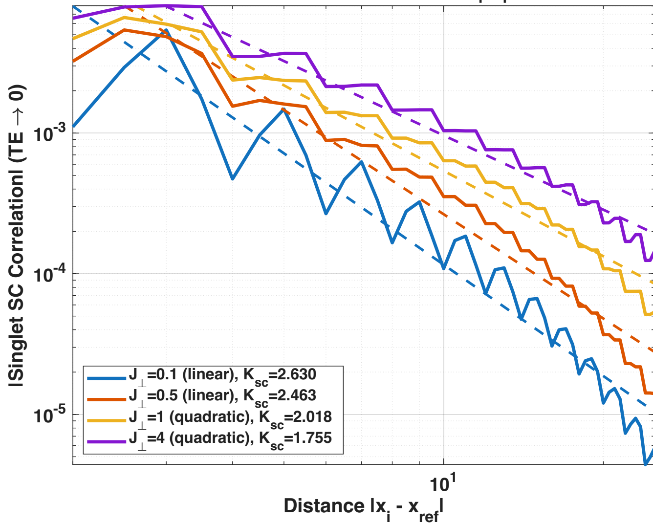
Extrapolated Singlet SC Correlations for J_{\perp\text{perp}} = 0.1, 0.5, 1, 4
