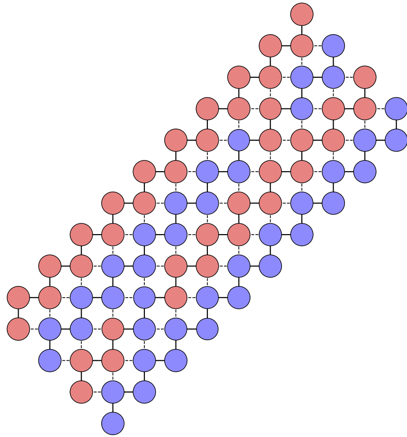
Layer 1 — localized spins
