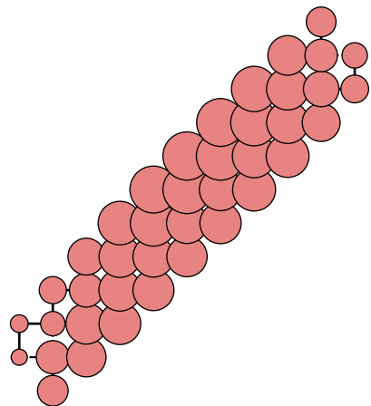
J_{\perp} = 0.1, D=6000
