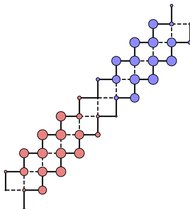
J_{\perp} = 0.3, \mathbf{D} = 6000
