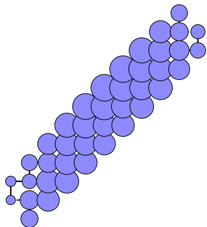
Layer 1 (localized)
