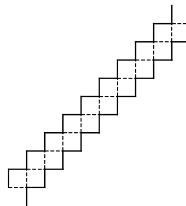
J_{\perp} = 0.5, \mathbf{D}=8000
