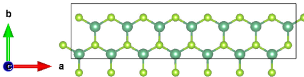
NbSe 2 supercell (as a part of misfit)
