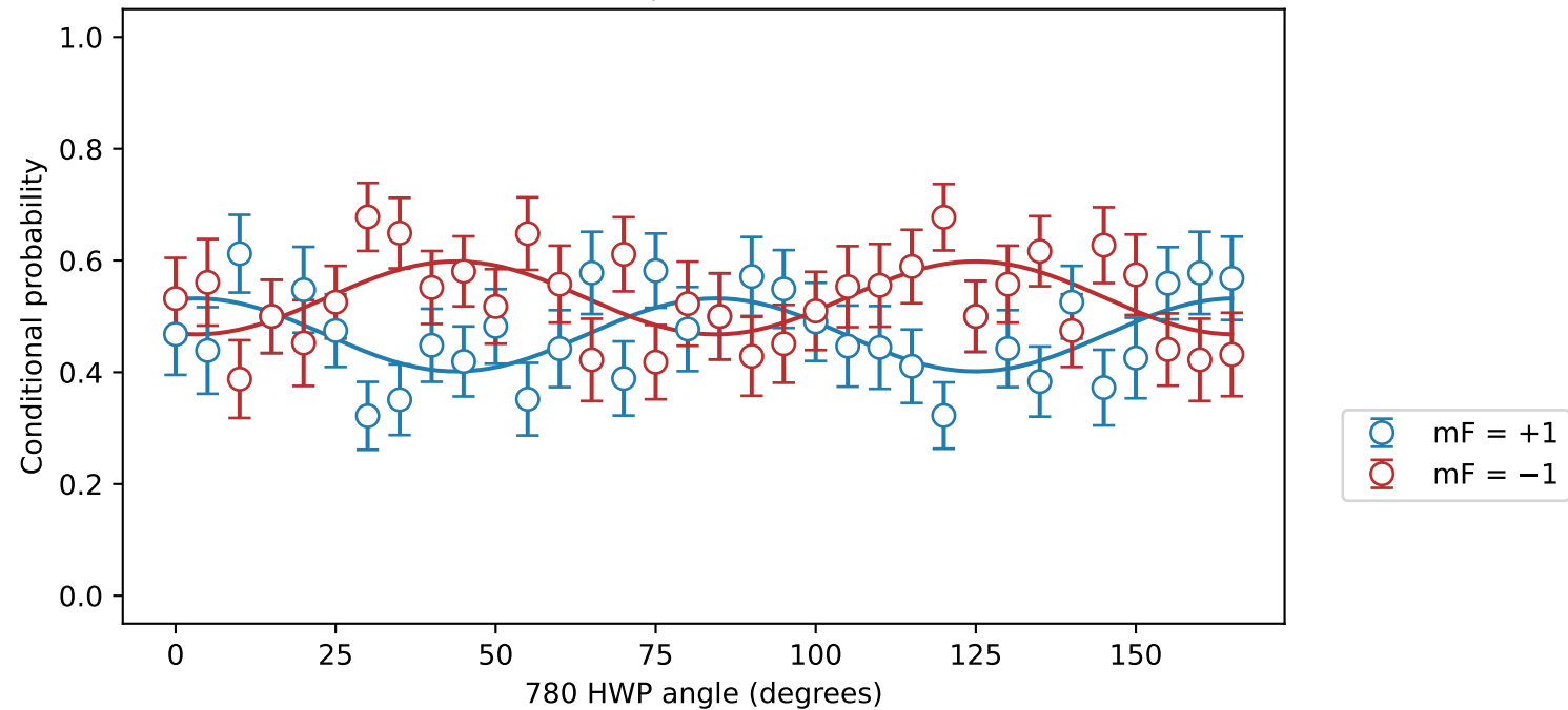
Atom state | SPCM0 detection
