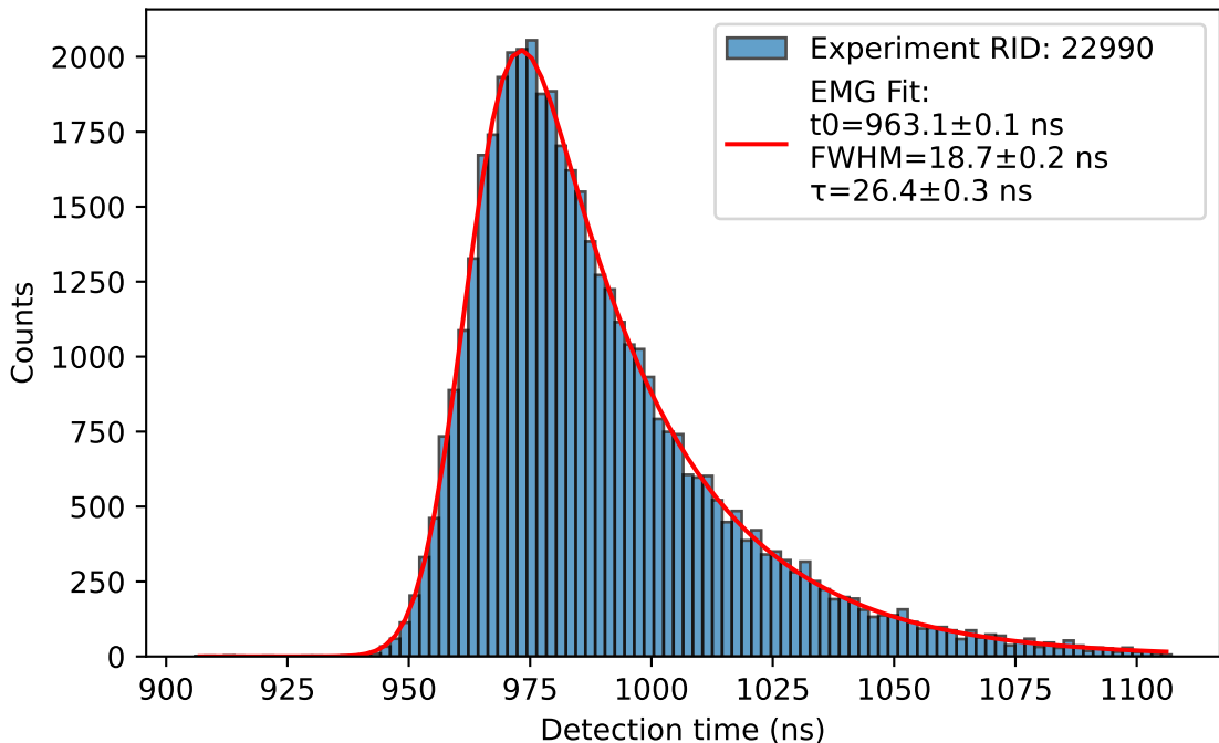
Photon Arrival Histogram: Gaussian Rise + Exponential Decay
