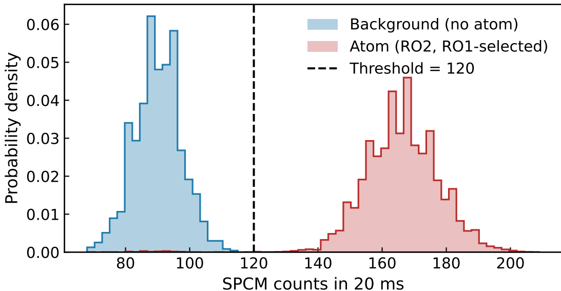
Single-atom readout histogram
