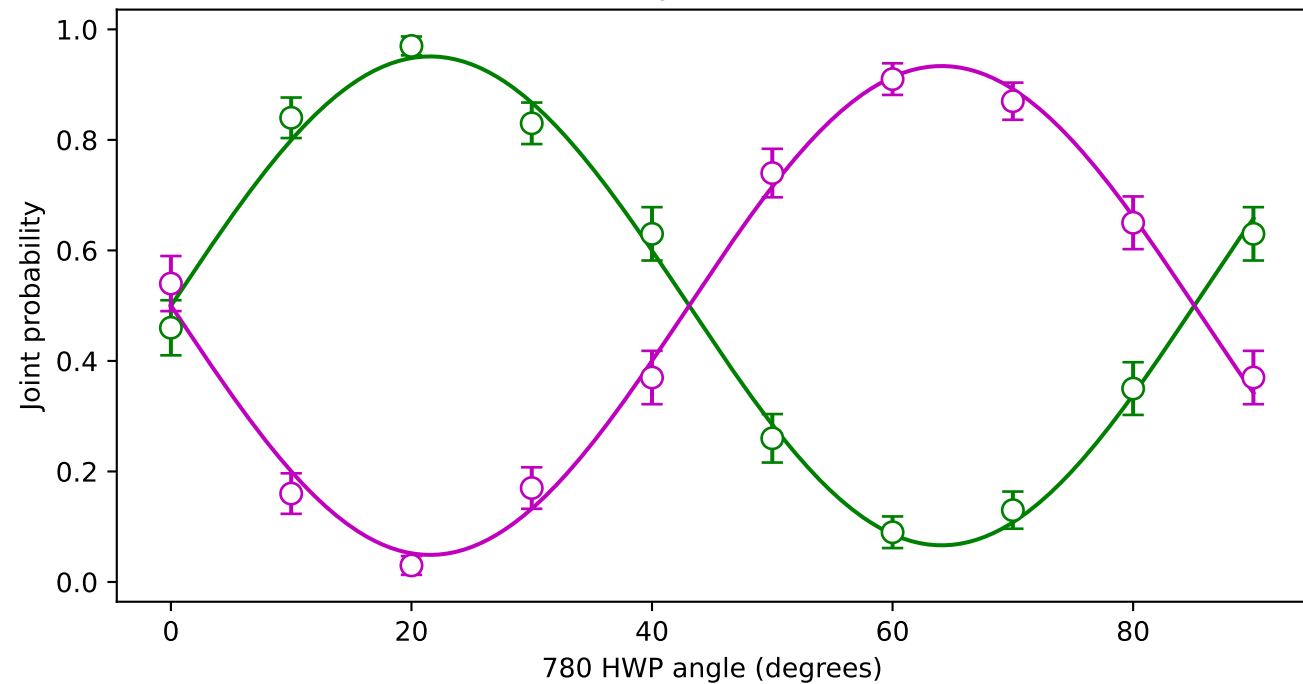
Parity-like sums
