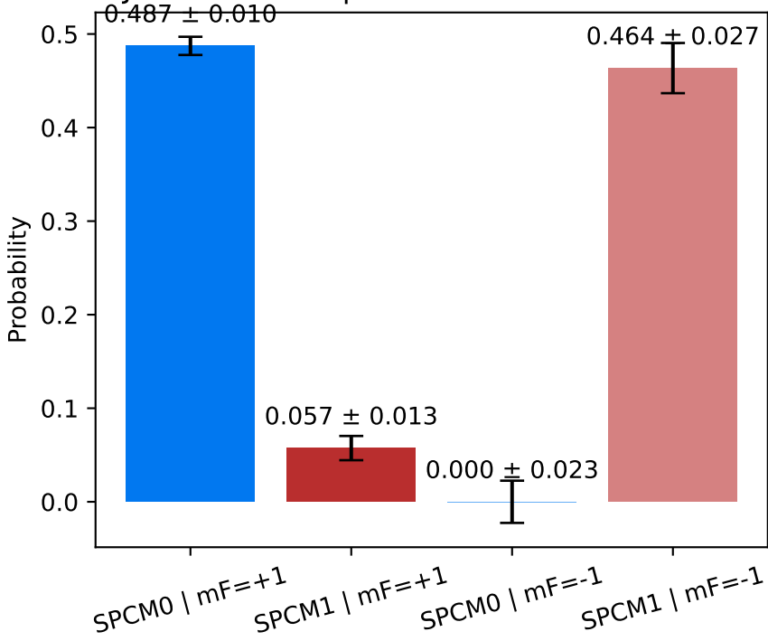
Joint detection probabilities at \theta^* = 21.51^\circ
