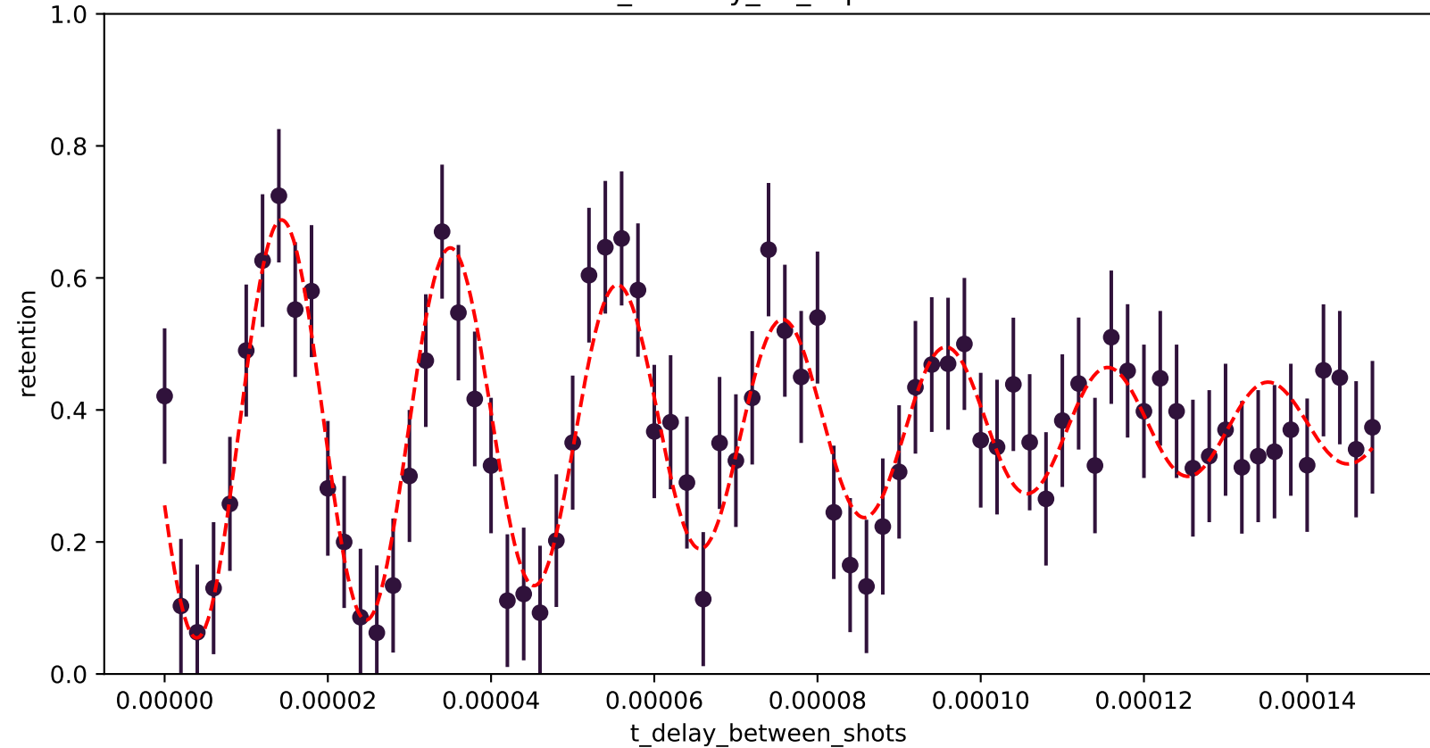
microwave_Ramsey_11_experiment 30559
