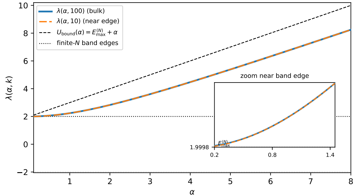
Defect eigenvalue \lambda(\alpha, k) vs. \alpha ( a = 0, b = 1, N = 200 )
