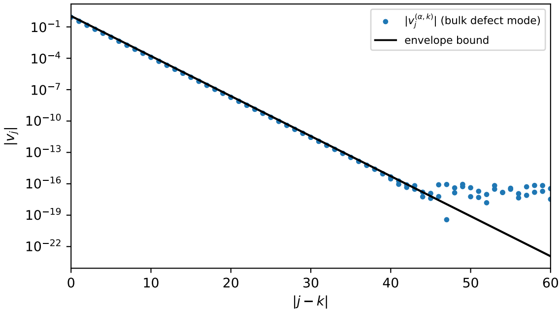
Semi-log localization at defect eigenvalue \lambda(\alpha, k) ( a = 0, b = 1, N = 200, k = 100, \alpha = 2 )
