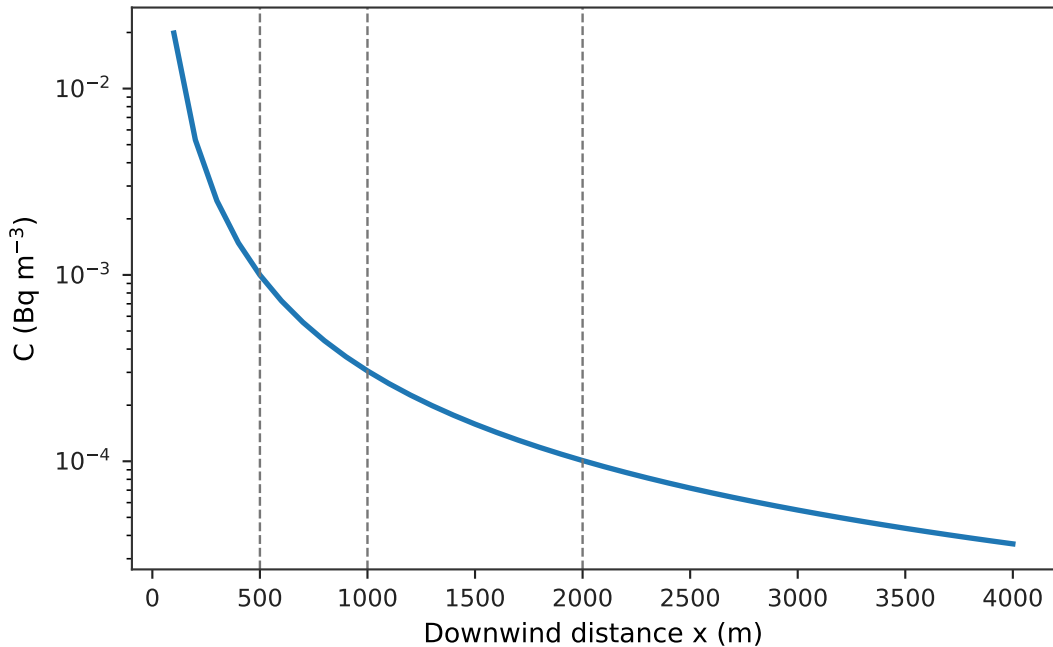
Centerline Concentration Profile
