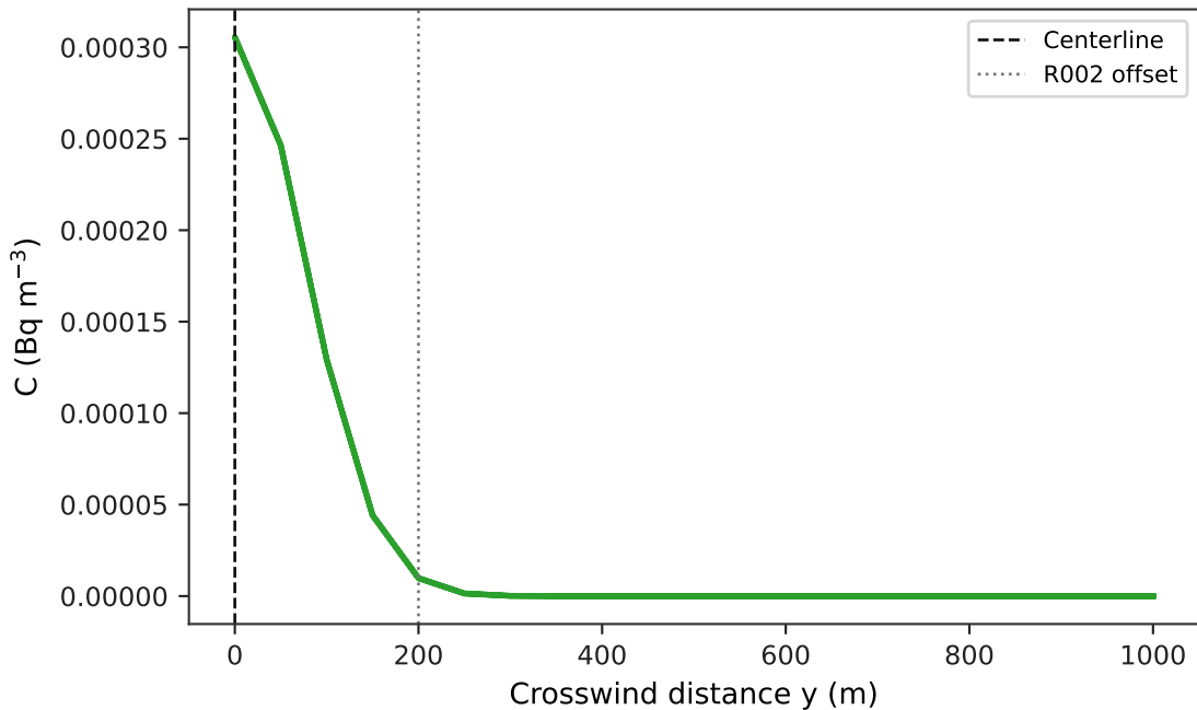
Crosswind Concentration Profile at x = 1000 m
