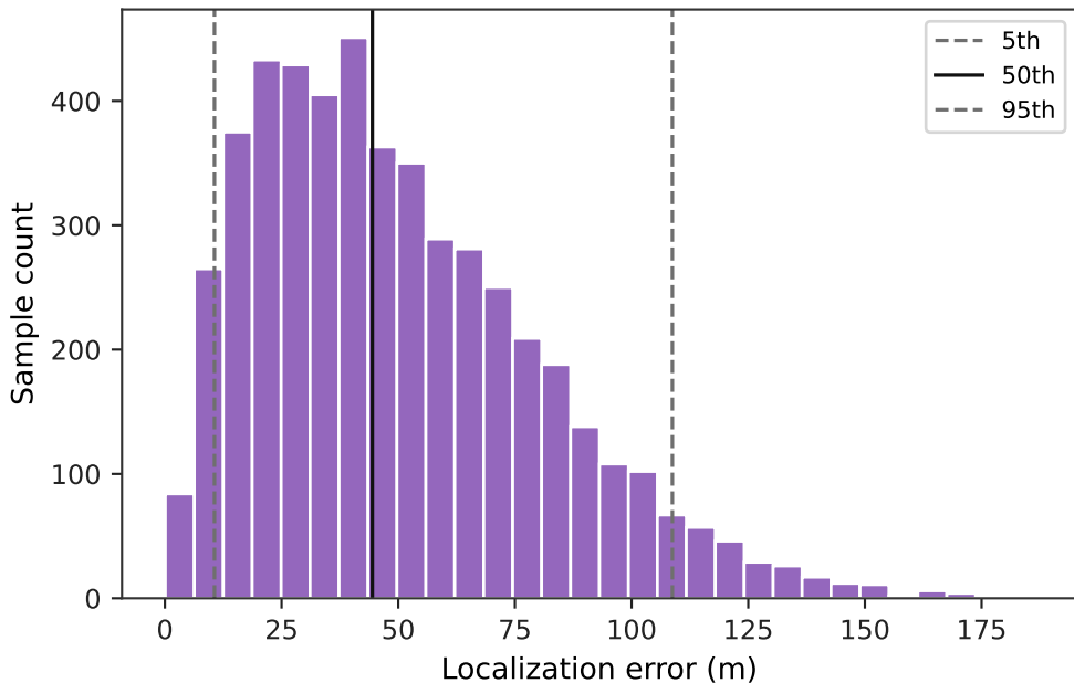
Monte Carlo Localization Error Distribution
