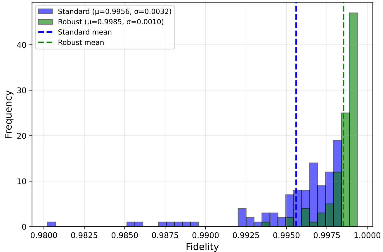
Fidelity Distribution over Ensemble (N=100)
