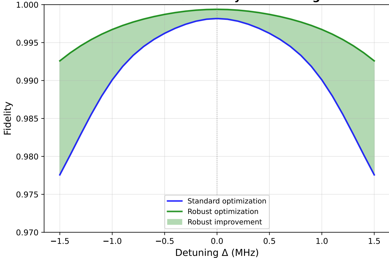
Robustness: Fidelity vs Detuning
