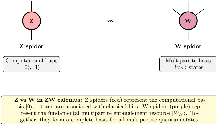
FIG. 26 Comparison of Z and W spiders in the ZW calculus. Z spiders encode classical bits in the computational basis, while W spiders provide the primitive for genuine multipartite entanglement. This dual representation enables complete characterization of quantum states.
