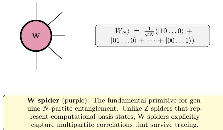
FIG. 24 The W spider in ZW calculus represents the N -partite W state. The W spider with N legs encodes the superposition where exactly one qubit is in state |1\rangle and the rest are |0\rangle , with all permutations equally weighted.
