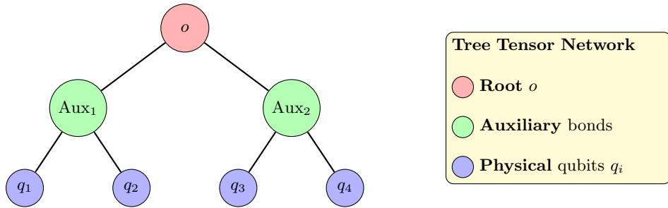
FIG. 19 Tree Tensor Network (TTN) representation of multipartite states. Physical qubits ( q_i ) are at the leaf nodes, while auxiliary bonds ( Aux_j ) encode the entanglement geometry. The bond dimension \chi controls the entanglement rank across each cut.
