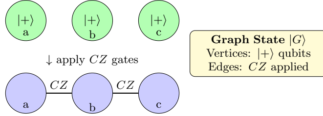
FIG. 10 Construction of a graph state from a graph G . Each vertex represents a qubit initialized in |+\rangle , and each edge represents a controlled- Z entangling operation applied between connected qubits.
