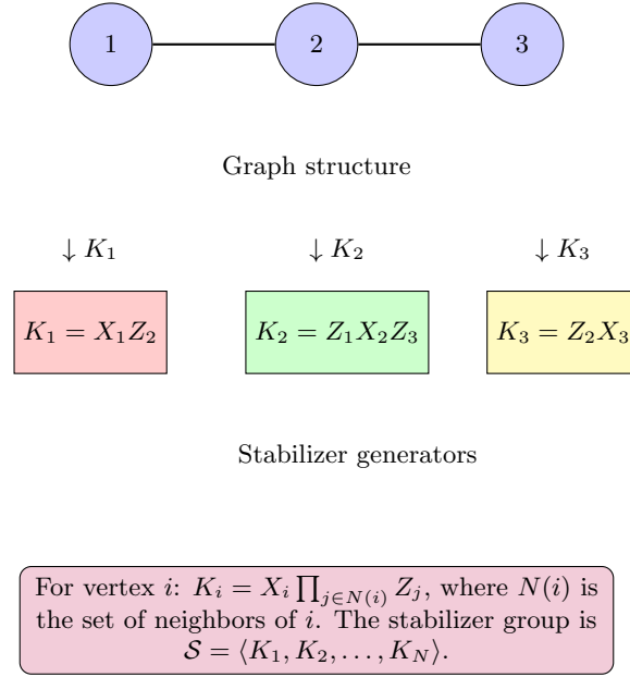
FIG. 14 Reading stabilizer generators from the graph structure. For each vertex i , the stabilizer generator K_i is the product of X on vertex i and Z on all its neighbors. These N operators generate the full stabilizer group of 2^N elements.
