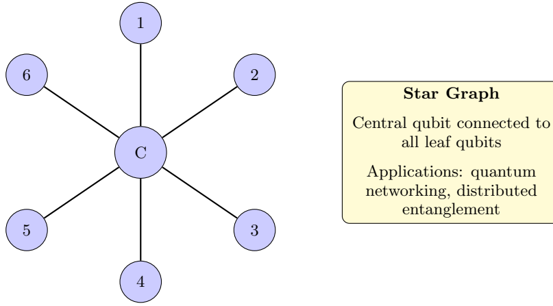
FIG. 12 Star graph configuration. The central qubit (C) is connected to all leaf qubits. Star graph states are highly symmetric and useful for quantum networking protocols where entanglement needs to be distributed from a central node.
