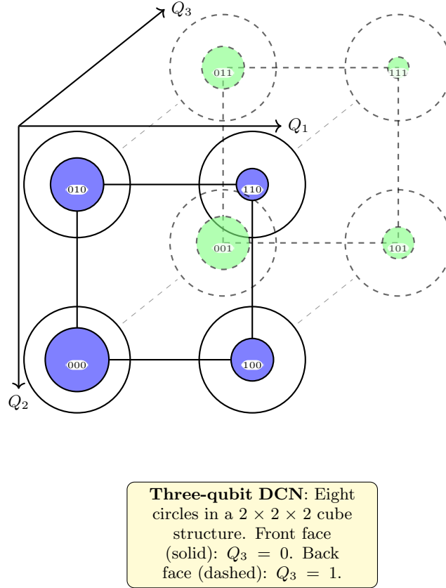
FIG. 4 Three-qubit state in Dimensional Circular Notation. The cube structure is shown with upright faces: front face ( Q_3 = 0 ) and back face ( Q_3 = 1 ) positioned top-right, each circle labeled by its basis state |Q_1Q_2Q_3\rangle .
