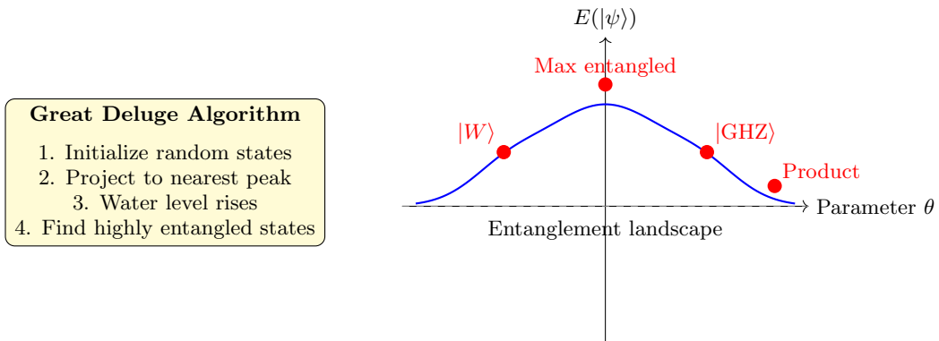
FIG. 9 Entanglement landscape visualization using the Great Deluge Algorithm. Peaks correspond to highly entangled states (GHZ, W), valleys to product states. The algorithm floods this landscape to identify maximally entangled configurations.
