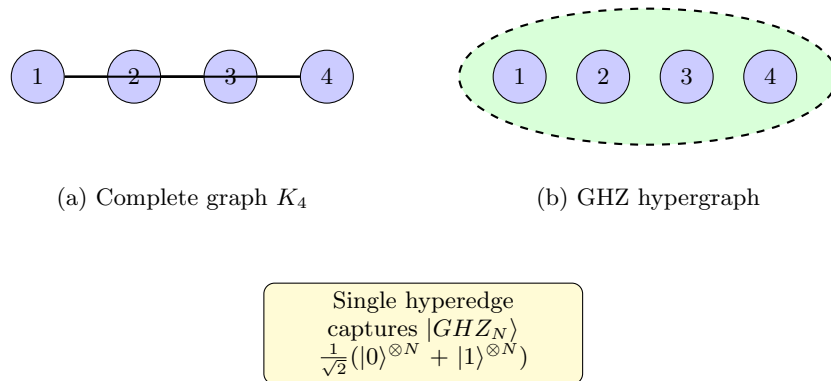
FIG. 17 GHZ state representation: (a) Complete graph K_4 requires many pairwise edges. (b) GHZ hypergraph represents the same state with a single hyperedge connecting all N qubits, capturing the genuine N -partite entanglement.
