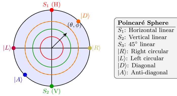
FIG. 7 Poincaré sphere representing polarization states of light. Each point on the sphere surface corresponds to a unique polarization state. For bipartite entanglement, composite Poincaré spheres can represent two-photon states.
