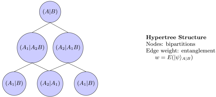
FIG. 8 Hypertree representation of multipartite entanglement. Each node represents a bipartition of the system, and edge weights quantify the entanglement across that cut. This hierarchical structure reveals the nesting of entanglement in tensor network states.
