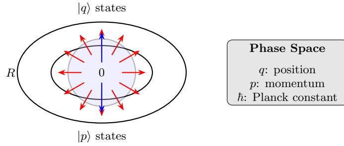
FIG. 5 Phase space representation for continuous-variable quantum systems. The torus structure arises from periodic boundary conditions in position ( q ) and momentum ( p ) spaces.
