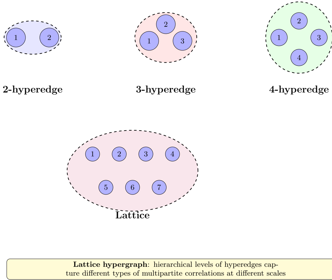
FIG. 18 Lattice hypergraph structure showing hierarchical levels. Different hyperedge sizes (2, 3, 4, N) capture correlations at different scales. The full lattice hypergraph combines all levels for complete characterization of multipartite entanglement.
