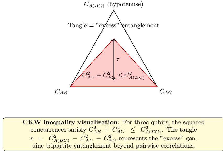
FIG. 30 Coffman-Kundu-Wootters (CKW) inequality visualization for three qubits. The triangle inequality shows that the squared entanglement C_{A(BC)}^2 (hypotenuse) must be at least as large as the sum of squared pairwise entanglements C_{AB}^2 + C_{AC}^2 . The tangle \tau represents the genuine tripartite entanglement not captured by pairwise measures.
