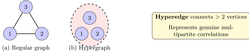
FIG. 16 Comparison of regular graphs and hypergraphs. In (a), each edge connects exactly two vertices, representing pairwise correlations. In (b), the dashed ellipse represents a hyperedge connecting three vertices, capturing genuine tripartite entanglement.
