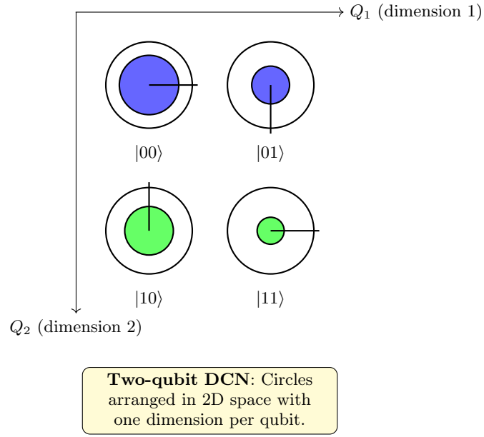
FIG. 3 Two-qubit state in Dimensional Circular Notation. Circles are arranged in a 2 \times 2 grid with explicit dimensional axes Q_1 and Q_2 , corresponding to the two qubits.
