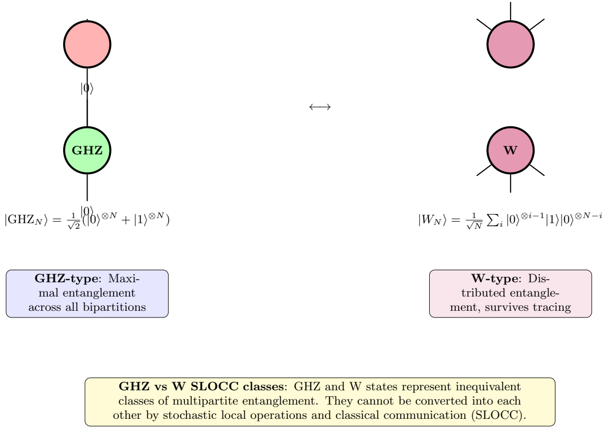
FIG. 25 Comparison of GHZ and W states in ZW calculus notation. GHZ states have maximal entanglement across all bipartitions, while W states have distributed entanglement that survives tracing out any single party. These represent distinct SLOCC equivalence classes for N \geq 3 .
