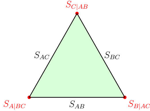
Figure 28: Triangle measure for three-qubit genuine multipartite entanglement. The one-to-other entropies S_{A|BC} , S_{B|AC} , S_{C|AB} form a triangle whose area is proportional to the squared tangle \tau . This connects geometric and entropic measures of entanglement.
