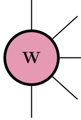
Figure 21: The W spider in ZW calculus represents the N -partite W state. The W spider with N legs encodes the superposition where exactly one qubit is in state |1\rangle and the rest are |0\rangle , with all permutations equally weighted.
