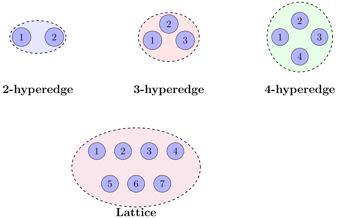
Figure 16: Lattice hypergraph structure showing hierarchical levels. Different hyperedge sizes (2, 3, 4, N ) capture correlations at different scales. The full lattice hypergraph combines all levels for complete characterization of multipartite entanglement.
