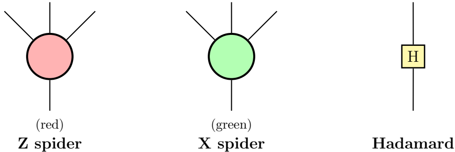
Figure 17: Basic elements of the ZX calculus: Z spiders (red, left), X spiders (green, center), and the Hadamard generator (yellow, right). Spiders are the fundamental building blocks representing quantum states and operations.
