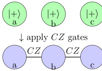
Figure 8: Construction of a graph state from a graph G . Each vertex represents a qubit initialized in |+\rangle , and each edge represents a controlled- Z entangling operation applied between connected qubits.
