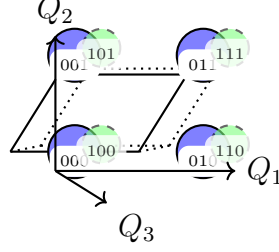
Figure 4: Three-qubit state in Dimensional Circular Notation, shown in isometric projection. The cube structure represents the three-dimensional arrangement corresponding to three qubits.
