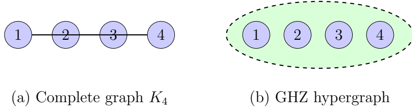
Figure 15: GHZ state representation: (a) Complete graph K_4 requires many pairwise edges. (b) GHZ hypergraph represents the same state with a single hyperedge connecting all N qubits, capturing the genuine N -partite entanglement.
