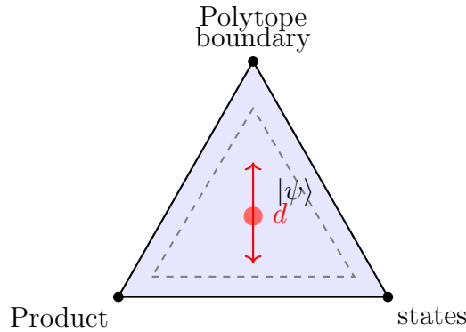
Figure 25: Entanglement polytope showing the position of a state |\psi\rangle within the polytope (2D projection). The distance d from the boundary indicates the amount of genuine multipartite entanglement.
