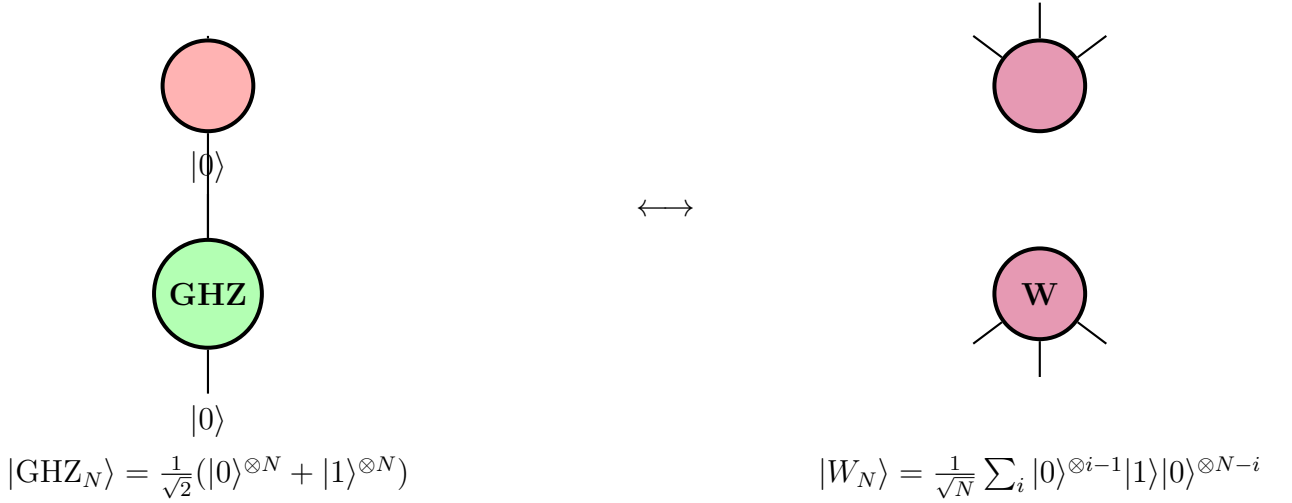
Figure 23: Comparison of GHZ and W states in ZW calculus notation. GHZ states have maximal entanglement across all bipartitions, while W states have distributed entanglement that survives tracing out any single party. These represent distinct SLOCC equivalence classes for N \geq 3 .
