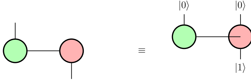
Figure 18: Bell state |\Phi^+\rangle representation in the ZX calculus. The green spider represents the |+\rangle state in the X basis, and connecting it to the red spider (in Z basis) creates the entangled Bell state.
