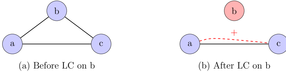
Figure 11: Illustration of local complementation on a graph state. When LC is applied to vertex b , an edge is added between its neighbors a and c . States related by LC (and edge additions/deletions) have equivalent entanglement structure. Local Complementation (LC): Applying LC on vertex v adds edges between all pairs of neighbors of v that weren't previously connected.
