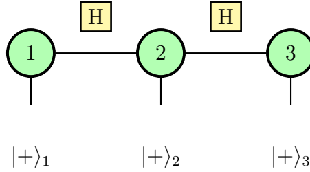
Figure 20: Graph state representation in ZX calculus. Three qubits prepared in |+\rangle (green spiders) are connected by Hadamard boxes (yellow), forming the graph state. The vertical wires represent the physical qubit outputs.
