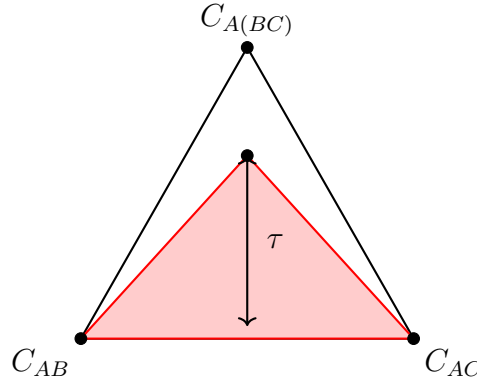
Figure 27: Coffman-Kundu-Wootters (CKW) inequality for three qubits. The squared entanglement C_{A(BC)}^2 (hypotenuse) must be at least as large as the sum C_{AB}^2 + C_{AC}^2 (base). The red region shows the tangle \tau , representing genuine tripartite entanglement not captured by pairwise measures.
