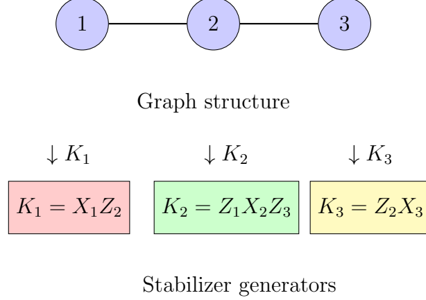
Figure 12: Reading stabilizer generators from the graph structure. For each vertex i , the stabilizer generator K_i is the product of X on vertex i and Z on all its neighbors. These N operators generate the full stabilizer group of 2^N elements. For vertex i : K_i = X_i \prod_{j \in N(i)} Z_j , where N(i) is the set of neighbors of i . The stabilizer group is \mathcal{S} = \langle K_1, K_2, \dots, K_N \rangle .
