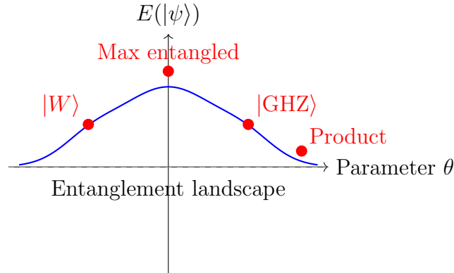
Figure 7: Entanglement landscape visualization using the Great Deluge Algorithm. Peaks correspond to highly entangled states (GHZ, W), valleys to product states. The algorithm floods this landscape to identify maximally entangled configurations. Great Deluge Algorithm: 1. Initialize random states, 2. Project to nearest peak, 3. Water level rises, 4. Find highly entangled states.
