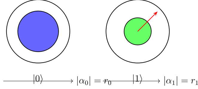
Figure 1: Single qubit state |\psi\rangle = \alpha_0|0\rangle + \alpha_1|1\rangle in Circle Representation. The filled inner circles represent amplitude magnitudes, while the red radial line in the right circle indicates the phase \phi relative to the |0\rangle state.
