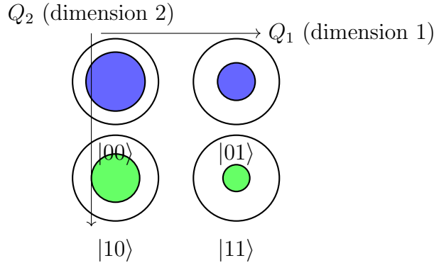
Figure 3: Two-qubit state in Dimensional Circular Notation. Circles are arranged in a 2 \times 2 grid with explicit dimensional axes Q_1 and Q_2 , corresponding to the two qubits.
