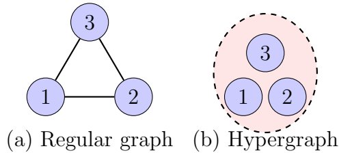
Figure 14: Comparison of regular graphs and hypergraphs. In (a), each edge connects exactly two vertices, representing pairwise correlations. In (b), the dashed ellipse represents a hyperedge connecting three vertices, capturing genuine tripartite entanglement.
