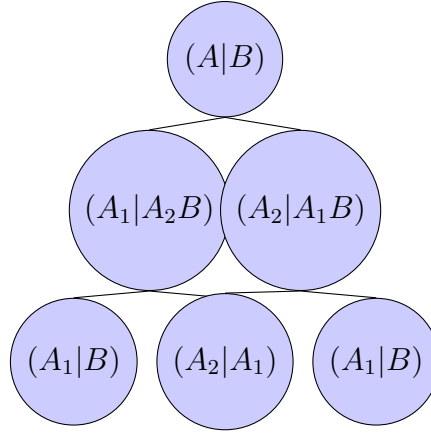
Figure 6: Hypertree representation of multipartite entanglement. Each node represents a bipartition of the system, and edge weights quantify the entanglement across that cut. This hierarchical structure reveals the nesting of entanglement in tensor network states. Hypertree Structure: Nodes = bipartitions, Edge weight = entanglement w = E(|\psi\rangle_{A|B}) .
