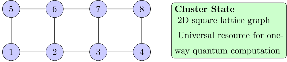
Grid of qubits with nearest-neighbor CZ entanglement
