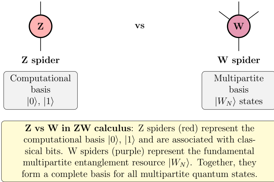
Figure 19: Comparison of Z and W spiders in the ZW calculus. Z spiders encode classical bits in the computational basis, while W spiders provide the primitive for genuine multipartite entanglement. This dual representation enables complete characterization of quantum states.
