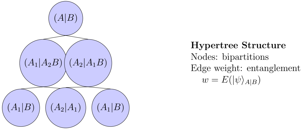
Figure 2: Hypertree representation of multipartite entanglement. Each node represents a bipartition of the system, and edge weights quantify the entanglement across that cut. This hierarchical structure reveals the nesting of entanglement in tensor network states.
