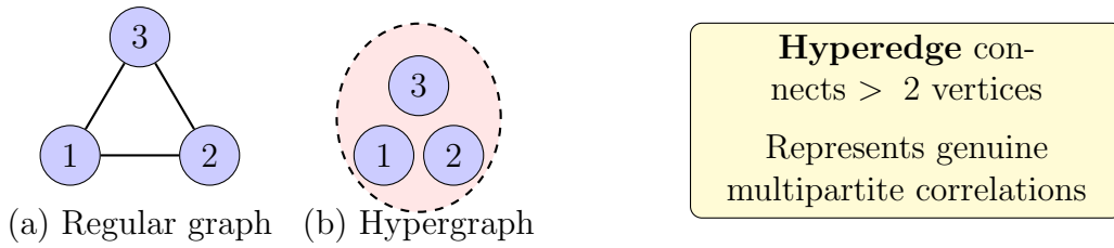
Figure 10: Comparison of regular graphs and hypergraphs. In (a), each edge connects exactly two vertices, representing pairwise correlations. In (b), the dashed ellipse represents a hyperedge connecting three vertices, capturing genuine tripartite entanglement.
