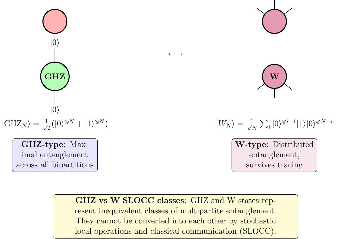
Figure 20: Comparison of GHZ and W states in ZW calculus notation. GHZ states have maximal entanglement across all bipartitions, while W states have distributed entanglement that survives tracing out any single party. These represent distinct SLOCC equivalence classes for N \geq 3 .
