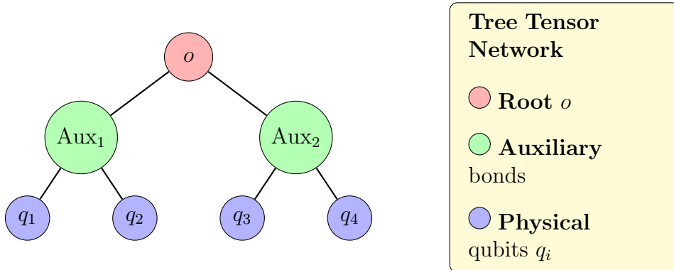
Figure 13: Tree Tensor Network (TTN) representation of multipartite states. Physical qubits ( q_i ) are at the leaf nodes, while auxiliary bonds ( Aux_j ) encode the entanglement geometry. The bond dimension \chi controls the entanglement rank across each cut.
