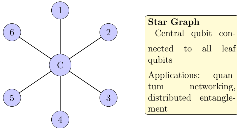
Figure 6: Star graph configuration. The central qubit (C) is connected to all leaf qubits. Star graph states are highly symmetric and useful for quantum networking protocols where entanglement needs to be distributed from a central node.
