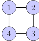
(c) Cycle C_4
