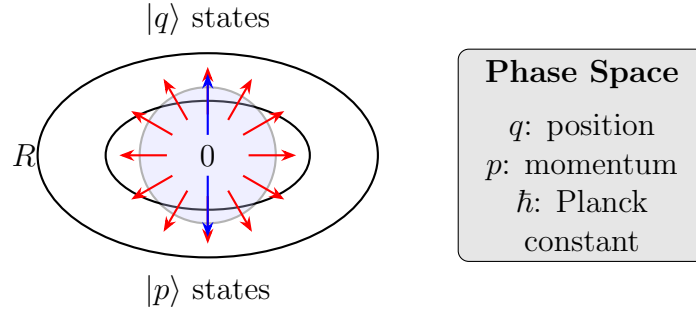
Figure 1: Phase space representation for continuous-variable quantum systems. The torus structure arises from periodic boundary conditions in position ( q ) and momentum ( p ) spaces.
