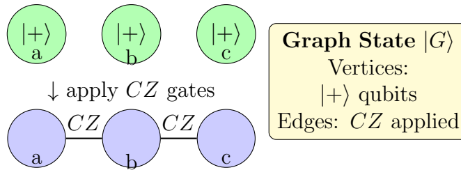
Figure 4: Construction of a graph state from a graph G . Each vertex represents a qubit initialized in |+\rangle , and each edge represents a controlled- Z entangling operation applied between connected qubits.
