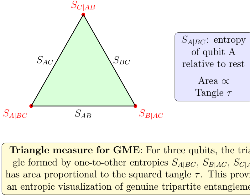
Figure 25: Triangle measure for three-qubit genuine multipartite entanglement. The one-to-other entropies S_{A|BC} , S_{B|AC} , S_{C|AB} form a triangle whose area is proportional to the squared tangle \tau . This connects geometric and entropic measures of entanglement.
