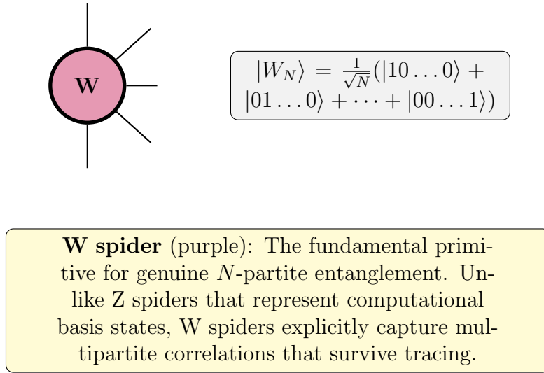
Figure 18: The W spider in ZW calculus represents the N -partite W state. The W spider with N legs encodes the superposition where exactly one qubit is in state |1\rangle and the rest are |0\rangle , with all permutations equally weighted.
