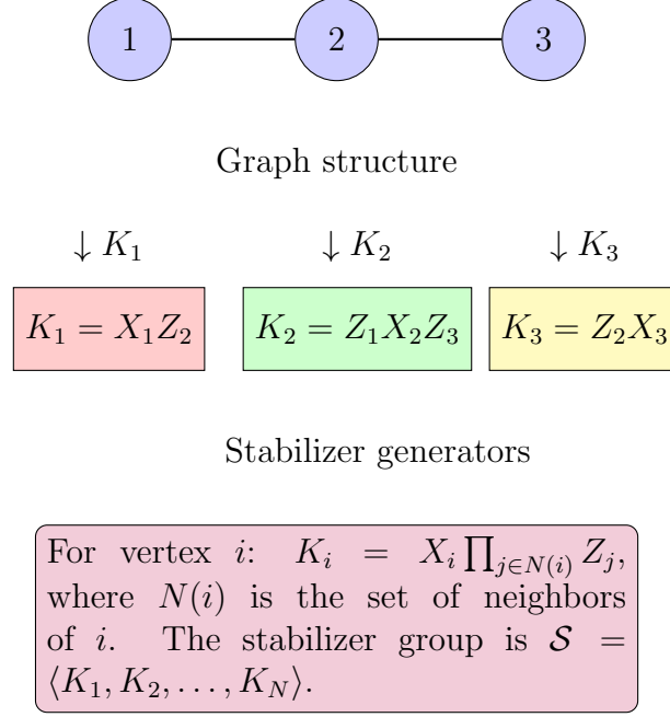
Figure 8: Reading stabilizer generators from the graph structure. For each vertex i , the stabilizer generator K_i is the product of X on vertex i and Z on all its neighbors. These N operators generate the full stabilizer group of 2^N elements.
