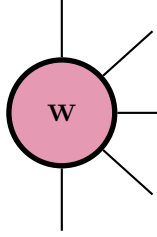
FIG. 30 The W spider in ZW calculus represents the N -partite W state. The W spider with N legs encodes the superposition where exactly one qubit is in state |1\rangle and the rest are |0\rangle , with all permutations equally weighted. W spider (purple): The fundamental primitive for genuine N -partite entanglement. Unlike Z spiders that represent computational basis states, W spiders explicitly capture multipartite correlations that survive tracing. |W_N\rangle = \frac{1}{\sqrt{N}}(|10\dots 0\rangle + |01\dots 0\rangle + \dots + |00\dots 1\rangle) .
