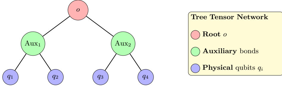
FIG. 25 Tree Tensor Network (TTN) representation of multipartite states. Physical qubits ( q_i ) are at the leaf nodes, while auxiliary bonds ( Aux_j ) encode the entanglement geometry. The bond dimension \chi controls the entanglement rank across each cut.
