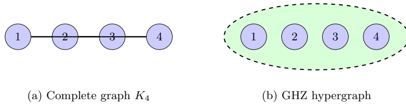
FIG. 23 GHZ state representation: (a) Complete graph K_4 requires many pairwise edges. (b) GHZ hypergraph represents the same state with a single hyperedge connecting all N qubits, capturing the genuine N -partite entanglement. Single hyperedge captures |GHZ_N\rangle = \frac{1}{\sqrt{2}}(|0\rangle^{\otimes N} + |1\rangle^{\otimes N}) .
