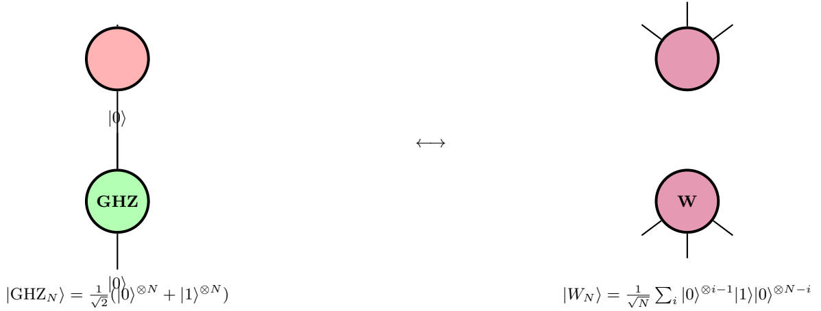
FIG. 31 Comparison of GHZ and W states in ZW calculus notation. GHZ states have maximal entanglement across all bipartitions, while W states have distributed entanglement that survives tracing out any single party. These represent distinct SLOCC equivalence classes for N \geq 3 . GHZ vs W SLOCC classes: GHZ and W states represent inequivalent classes of multipartite entanglement. They cannot be converted into each other by stochastic local operations and classical communication (SLOCC). GHZ-type: Maximal entanglement across all bipartitions. W-type: Distributed entanglement, survives tracing.
