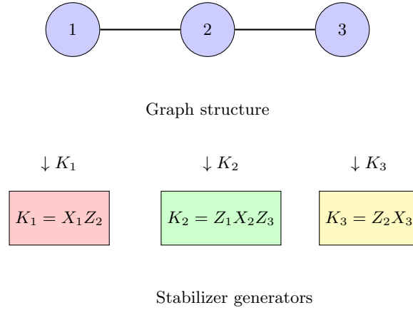
FIG. 20 Reading stabilizer generators from the graph structure. For each vertex i , the stabilizer generator K_i is the product of X on vertex i and Z on all its neighbors. These N operators generate the full stabilizer group of 2^N elements. For vertex i : K_i = X_i \prod_{j \in N(i)} Z_j , where N(i) is the set of neighbors of i . The stabilizer group is \mathcal{S} = \langle K_1, K_2, \dots, K_N \rangle .
