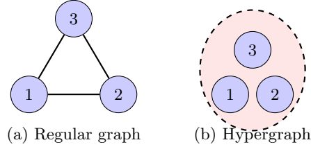
FIG. 22 Comparison of regular graphs and hypergraphs. In (a), each edge connects exactly two vertices, representing pairwise correlations. In (b), the dashed ellipse represents a hyperedge connecting three vertices, capturing genuine tripartite entanglement. Hyperedge connects > 2 vertices and represents genuine multipartite correlations.
