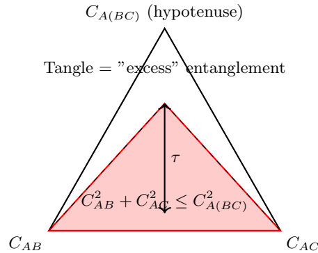
FIG. 36 Coffman-Kundu-Wootters (CKW) inequality visualization for three qubits. The triangle inequality shows that the squared entanglement C_{A(BC)}^2 (hypotenuse) must be at least as large as the sum of squared pairwise entanglements C_{AB}^2 + C_{AC}^2 . The tangle \tau represents the genuine tripartite entanglement not captured by pairwise measures. CKW inequality visualization: For three qubits, the squared concurrences satisfy C_{AB}^2 + C_{AC}^2 \leq C_{A(BC)}^2 . The tangle \tau = C_{A(BC)}^2 - C_{AB}^2 - C_{AC}^2 represents the "excess" genuine tripartite entanglement beyond pairwise correlations.
