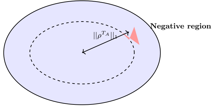
FIG. 35 Negativity visualization: the partial transpose \rho^{TA} of an entangled state has negative eigenvalues (shown in red). The negativity N(\rho) measures the total "volume" of these negative regions, providing a quantifier of bipartite entanglement. Negativity N(\rho) = \frac{\|\rho^{TA}\|_1 - 1}{2} : The "volume" of negative eigenvalues in the partial transpose indicates entanglement. For separable states, all eigenvalues are positive; for entangled states, negative eigenvalues appear.
