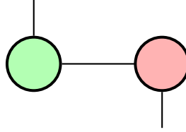
FIG. 27 Bell state |\Phi^+\rangle representation in the ZX calculus. The green spider represents the |+\rangle state in the X basis, and connecting it to the red spider (in Z basis) creates the entangled Bell state. Bell state in ZX: A green spider with two outputs connected to a red spider with two inputs represents the maximally entangled Bell state |\Phi^+\rangle = \frac{1}{\sqrt{2}}(|00\rangle + |11\rangle) .
