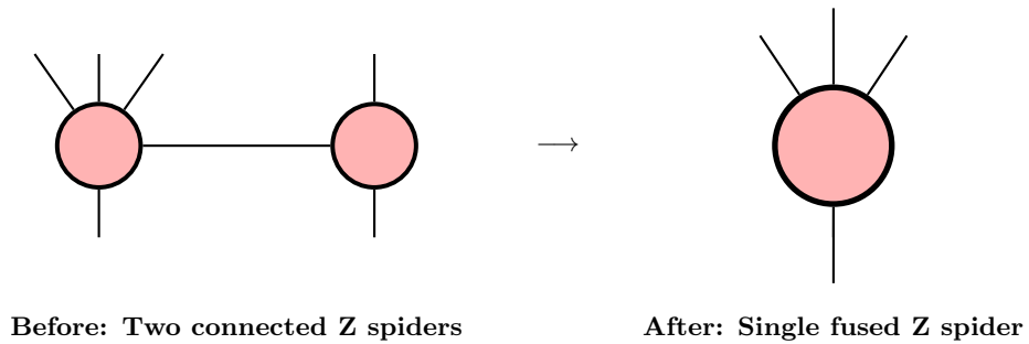
FIG. 28 The Spider Theorem in ZX calculus: two connected Z spiders fuse into a single Z spider. This fundamental rule enables simplification of ZX diagrams and reasoning about quantum operations. Spider Theorem (Fusion): When two spiders of the same color are connected, they fuse into a single spider. The total number of wires is preserved: (m, n) \cup (n, p) = (m, p) .
