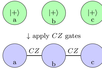
FIG. 16 Construction of a graph state from a graph G . Each vertex represents a qubit initialized in |+\rangle , and each edge represents a controlled- Z entangling operation applied between connected qubits. Graph State |G\rangle : Vertices = |+\rangle qubits, Edges = CZ applied.
