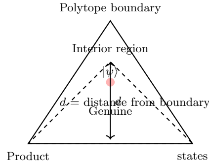
FIG. 34 Entanglement polytope showing the position of a state |\psi\rangle within the polytope. The distance from the boundary indicates the amount of genuine multipartite entanglement. Extreme points (vertices) correspond to product states, while the interior contains genuinely multipartite entangled states. Entanglement vector position: A state's position within the polytope indicates its entanglement. The distance d from the boundary measures how "genuinely" entangled the state is. States near the boundary have less genuine multipartite entanglement.
