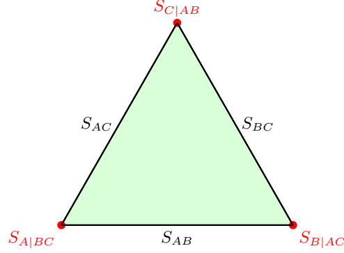
FIG. 37 Triangle measure for three-qubit genuine multipartite entanglement. The one-to-other entropies S_{A|BC} , S_{B|AC} , S_{C|AB} form a triangle whose area is proportional to the squared tangle \tau . This connects geometric and entropic measures of entanglement. Triangle measure for GME: For three qubits, the triangle formed by one-to-other entropies has area proportional to the squared tangle \tau . S_{A|BC} = entropy of qubit A relative to rest, \text{Area} \propto \text{Tangle } \tau .
