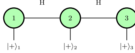
FIG. 29 Graph state representation in ZX calculus. Three qubits prepared in |+\rangle (green spiders) are connected by Hadamard boxes (yellow), forming the graph state. The vertical wires represent the physical qubit outputs. Graph state |G\rangle : Green spiders = graph vertices, H boxes = edges, Vertical wires = qubit outputs. Graph state in ZX: Each vertex is a green spider prepared in |+\rangle . Edges are represented by Hadamard boxes connecting the spiders, implementing the CZ entangling operation.
