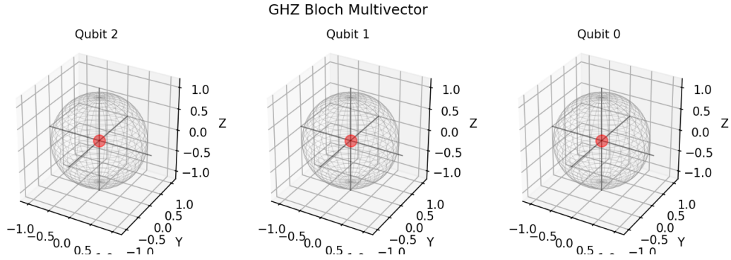
FIG. 14 Bloch Multivector visualization of the 3-qubit GHZ state |\text{GHZ}_3\rangle . Three Bloch spheres show the reduced state of each qubit. For the GHZ state, all qubits are maximally mixed ( \rho_i = I/2 ), indicating maximal entanglement.
