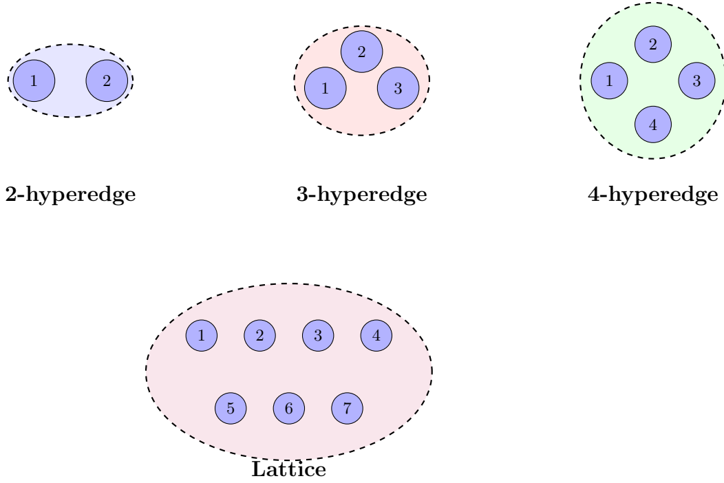
FIG. 24 Lattice hypergraph structure showing hierarchical levels. Different hyperedge sizes (2, 3, 4, N) capture correlations at different scales. The full lattice hypergraph combines all levels for complete characterization of multipartite entanglement. Lattice hypergraph: hierarchical levels of hyperedges capture different types of multipartite correlations at different scales.
