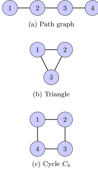
FIG. 21 Different graph representations of the GHZ state. The GHZ state can be represented as a path graph, cycle graph, or other connected structures, all of which are locally complemented to each other and thus share equivalent entanglement properties. GHZ state equivalence: |\text{GHZ}_N\rangle = \frac{1}{\sqrt{2}}(|0\rangle^{\otimes N} + |1\rangle^{\otimes N}) can be represented by different graph structures that are LC-equivalent (connected through local complementations).
