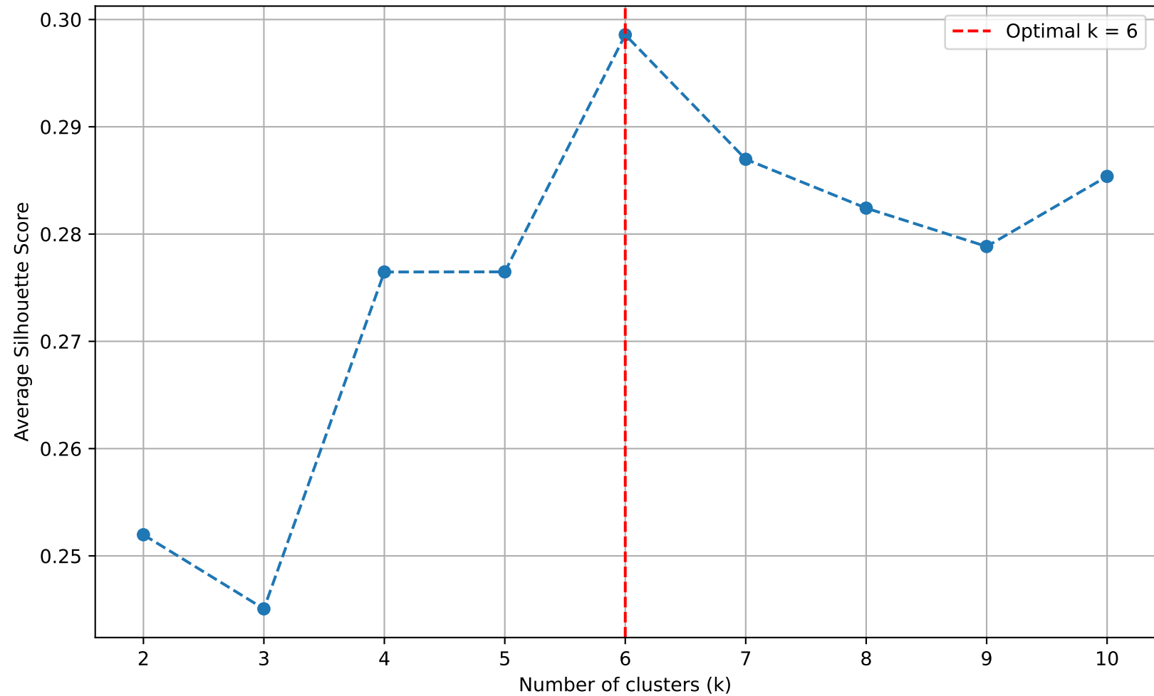
Silhouette Scores for Optimal k
