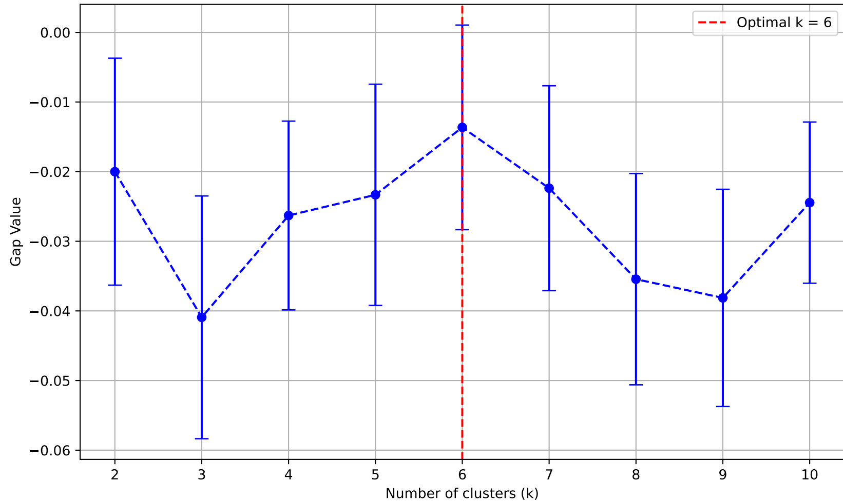
Gap Statistic for Optimal k
