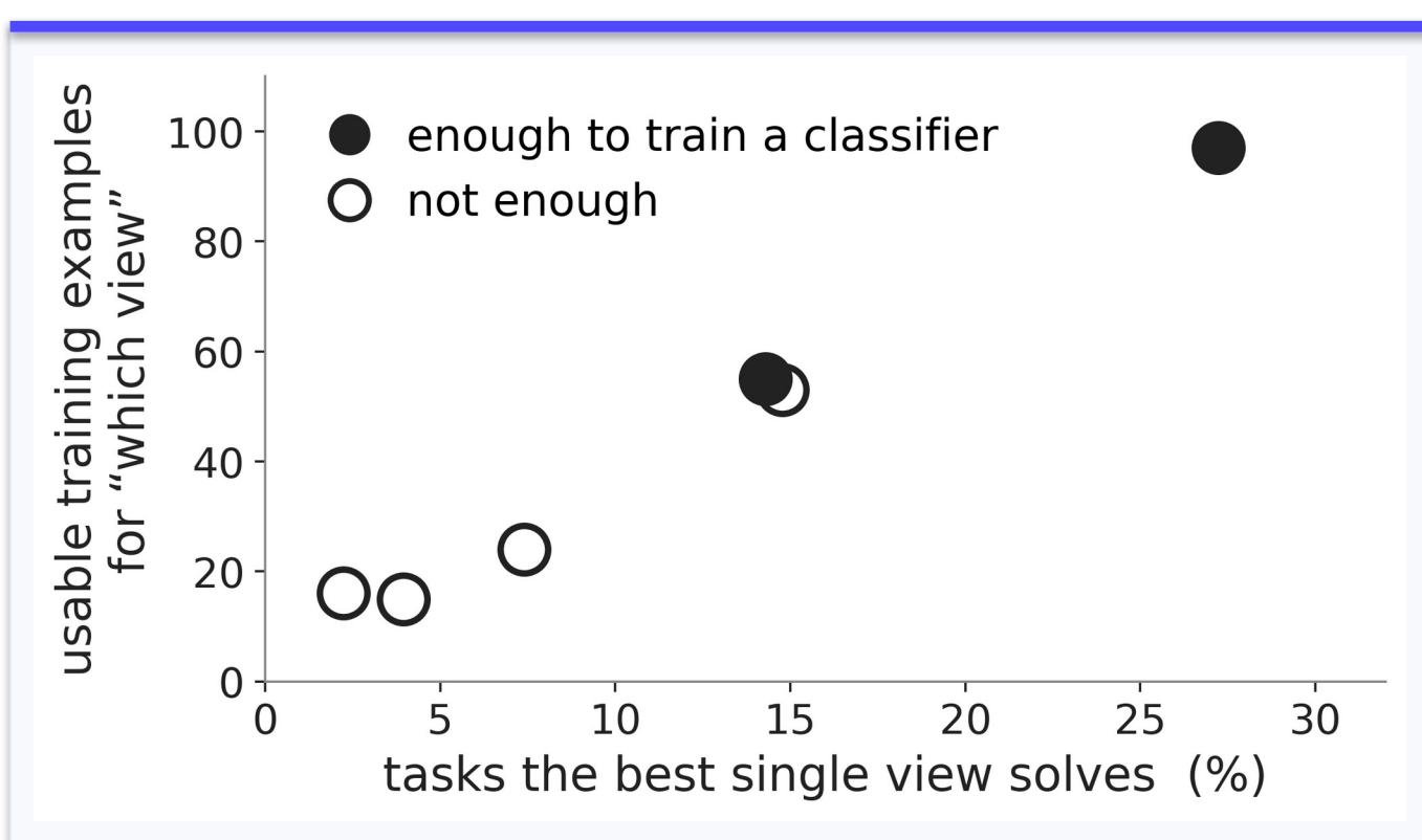
Fig 3. Usable “which view” examples against the best single view’s success rate, one point per VisualWebArena setting. Examples exist only where tasks get solved.
