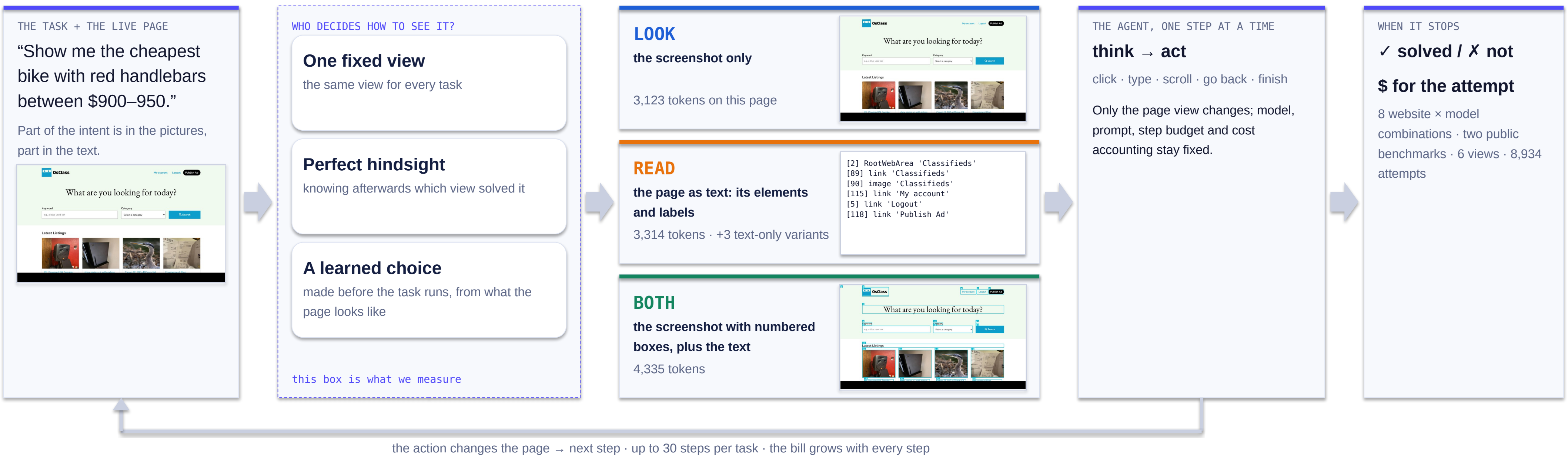
Fig 1. Everything is held fixed except how the page is shown. The dashed box is what this work measures — one fixed view, perfect hindsight, or a choice a model had to learn — each judged on both success and cost. The laptop beside this poster replays the loop on three tasks.
