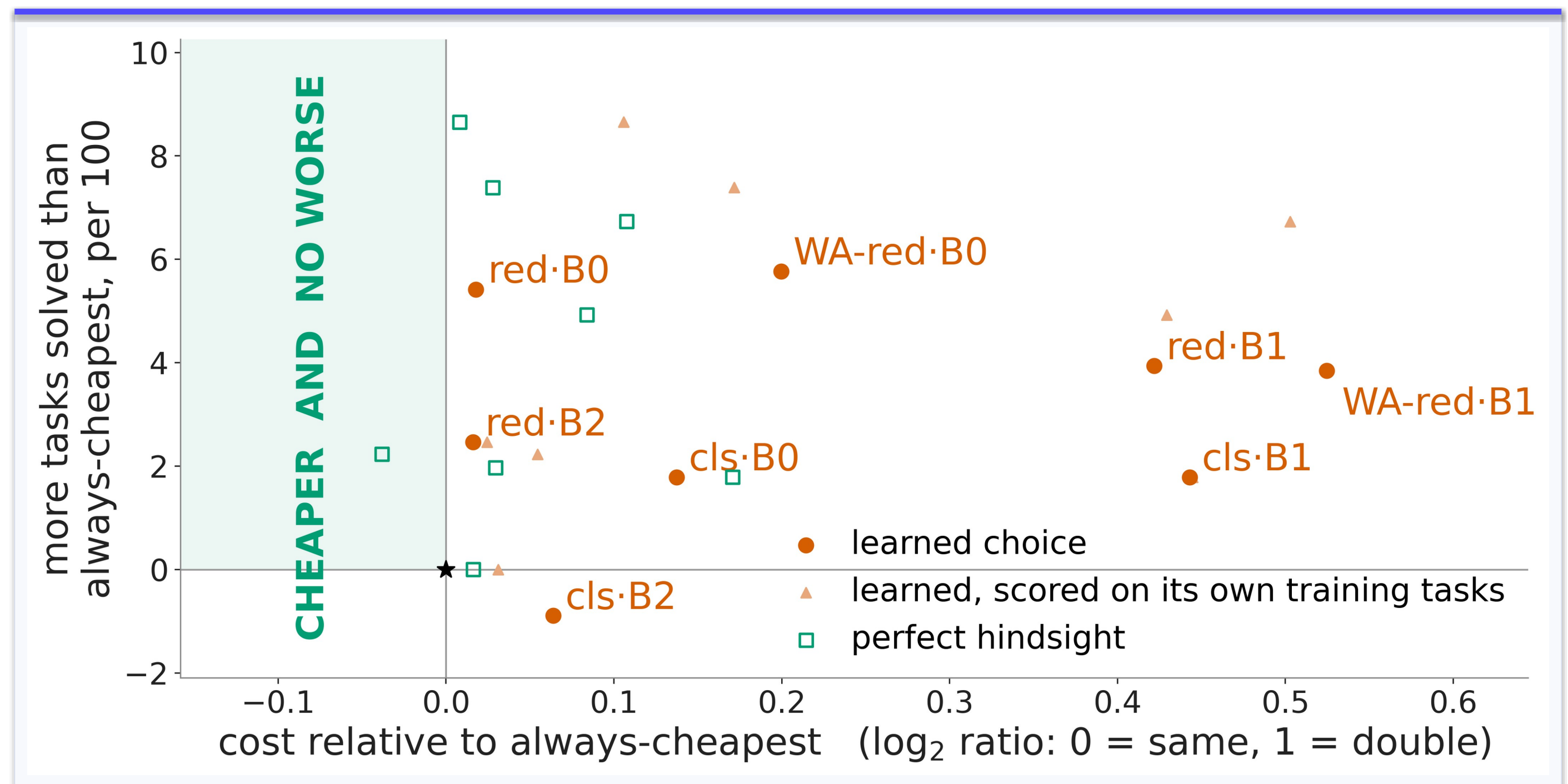
Fig 2. Every way of choosing a view, in every setting, compared with one fixed rule: always use the cheapest view (★). A win lands in the shaded region — cheaper and no worse. Always-cheapest is cheapest on average, not on every task, which is why a few points sit left of it. Learned choices are scored only on tasks they never saw.
