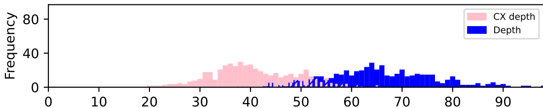
SAT
