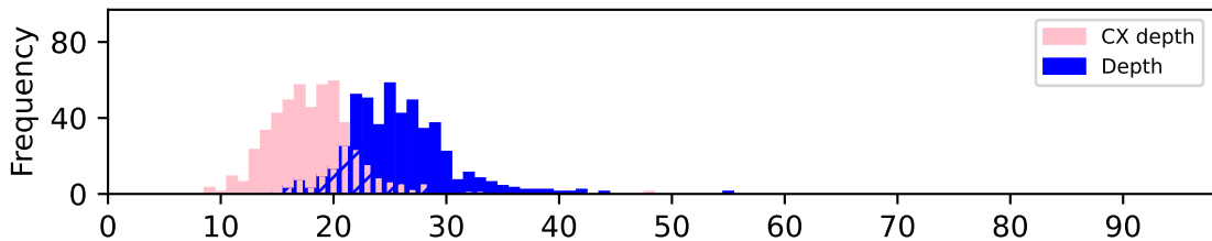
Greedy
