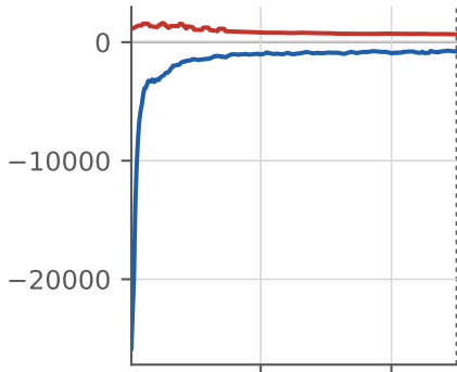
micro_segmented
