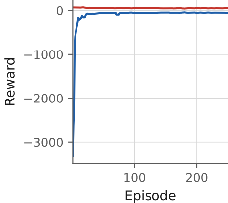
dmz
