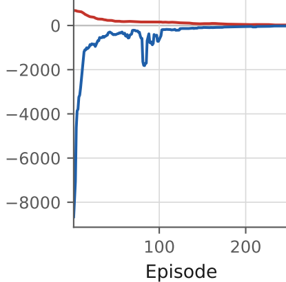
micro_segmented
