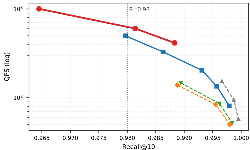
Deep-96-angular (learned CNN embeddings)
