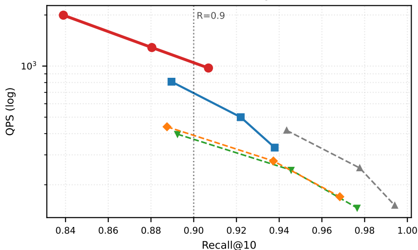
GloVe-200-angular (word vectors, angular)
