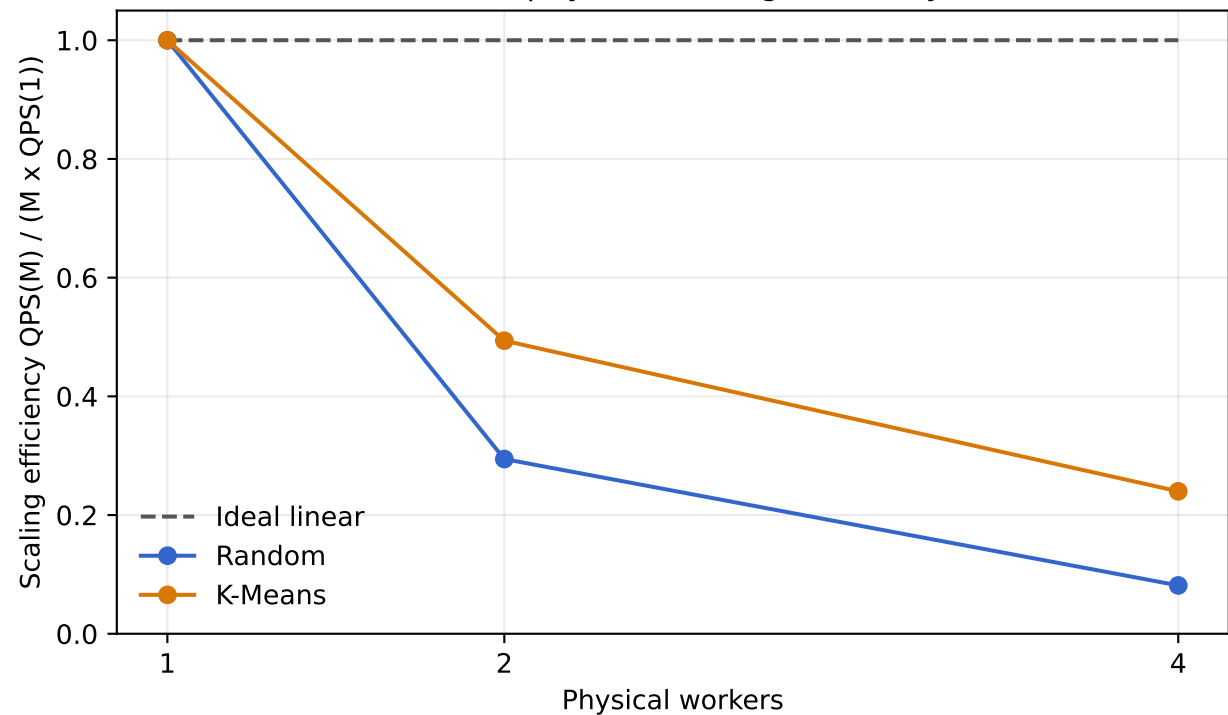
SIFT1M physical scaling efficiency
