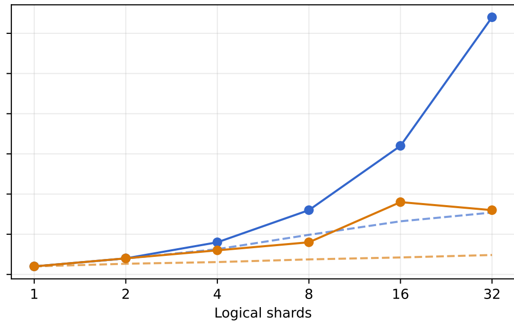
GloVe-200-angular
