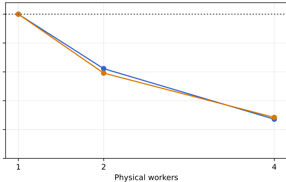
GloVe-200-angular
