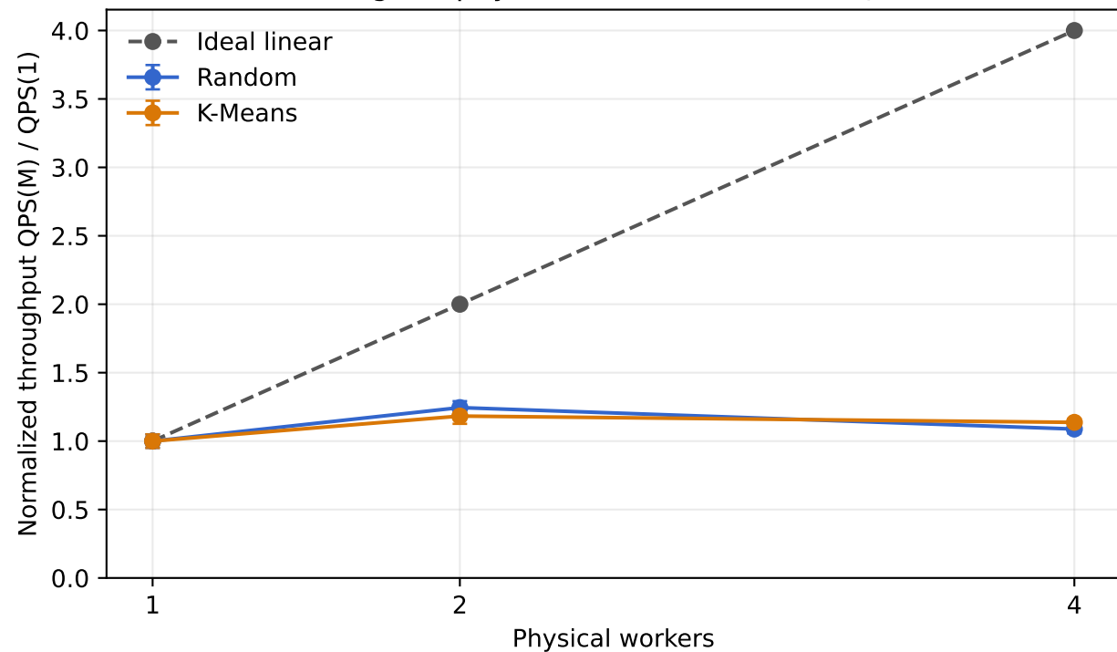
GloVe-200-angular physical scale-out at Recall@10 \geq 0.90
