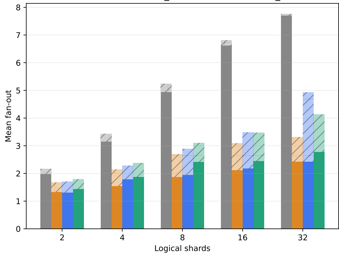
GloVe-200: solid P_exact + hatched Delta_P
