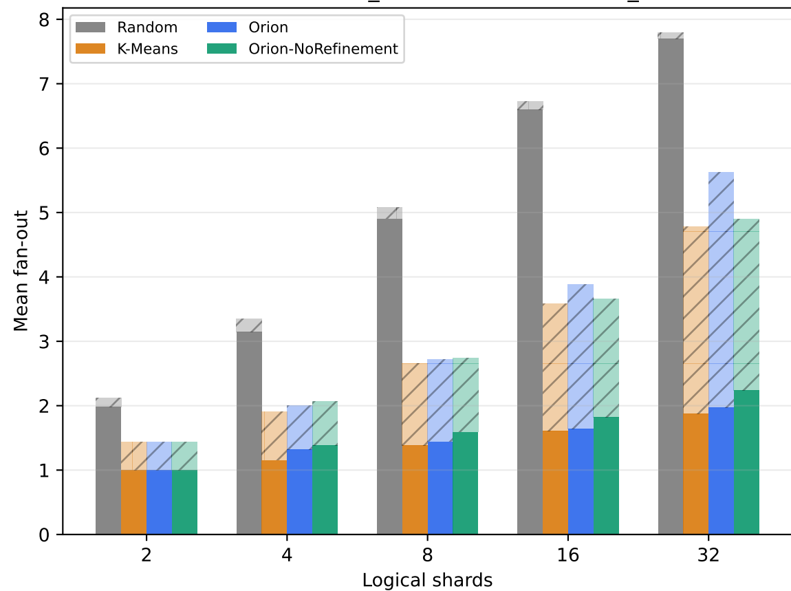
SIFT1M: solid P_exact + hatched Delta_P
