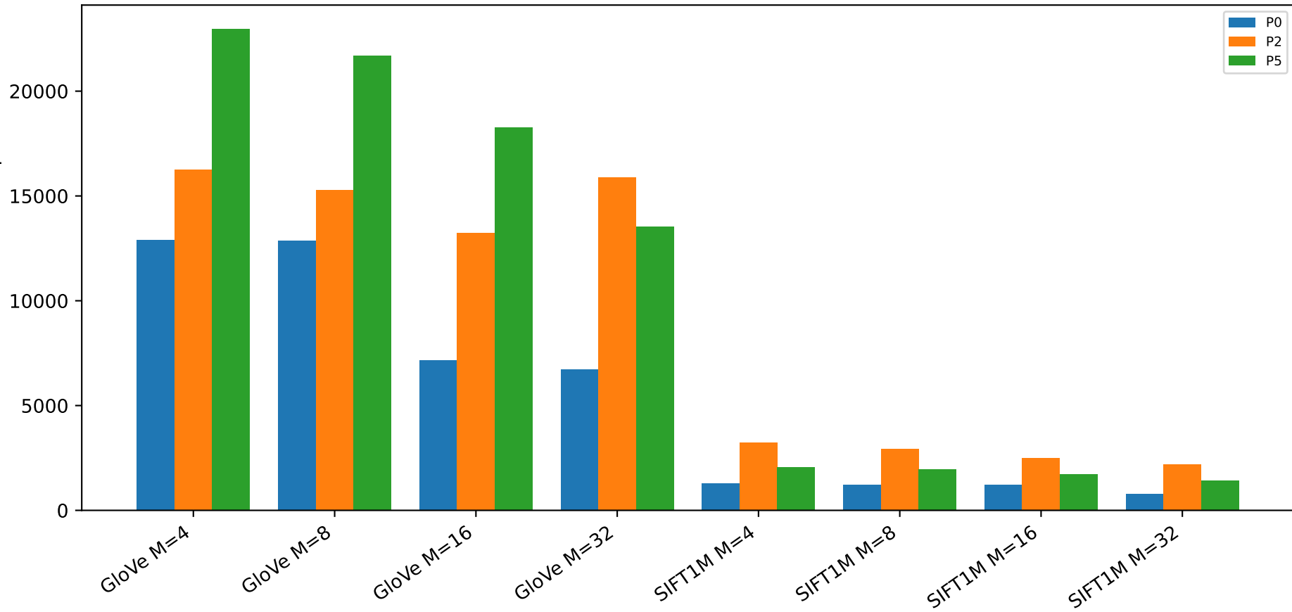
P95 max-shard distance computations
