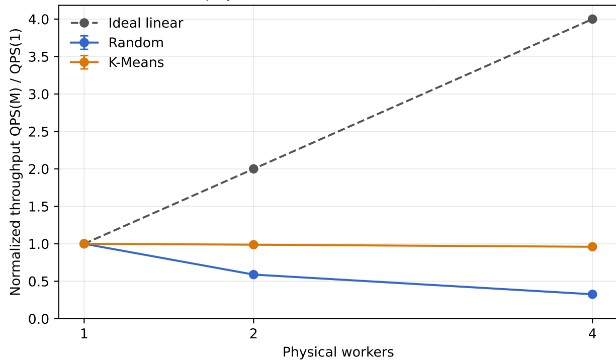
SIFT1M physical scale-out at Recall@10 \geq 0.90
