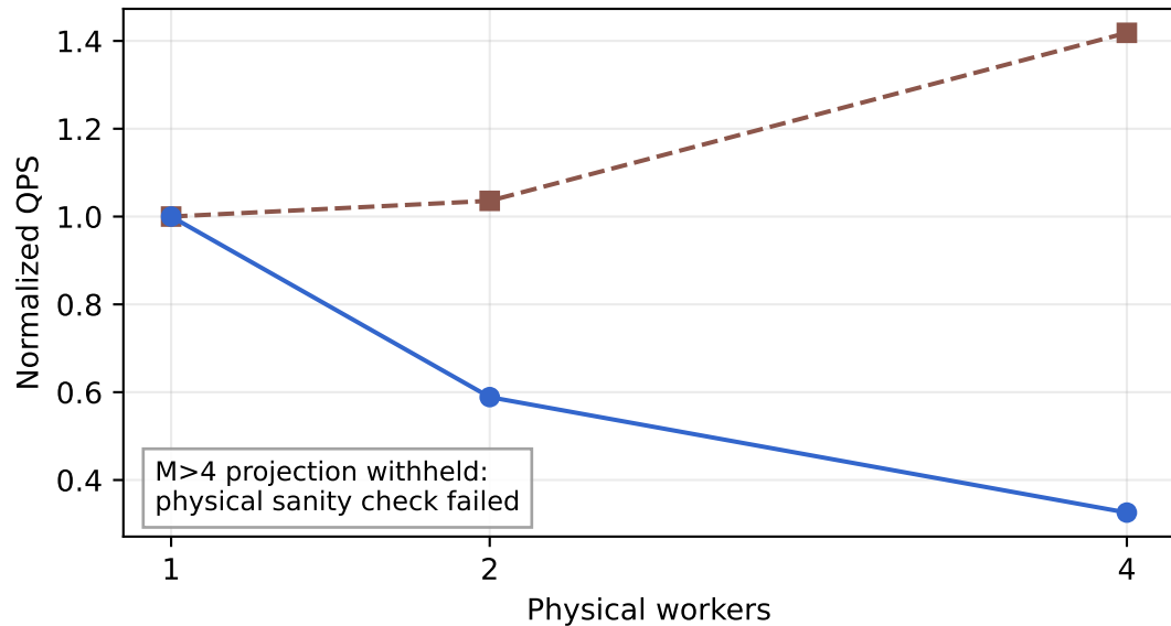
Random
