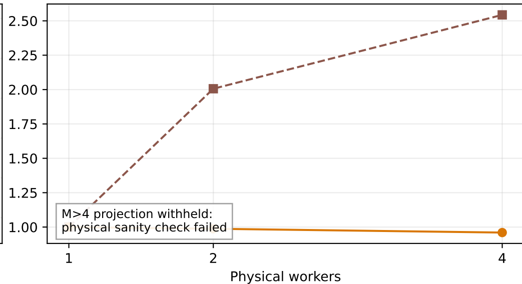
K-Means
