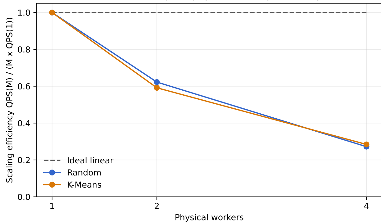
GloVe-200-angular physical scaling efficiency
