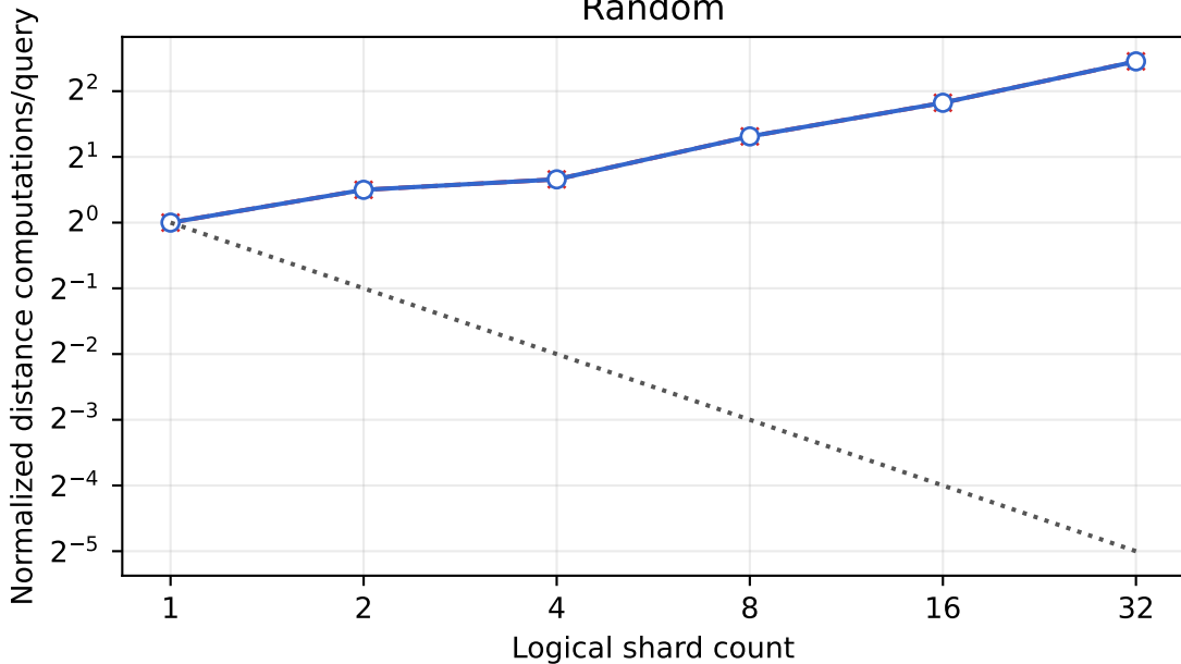
Random
