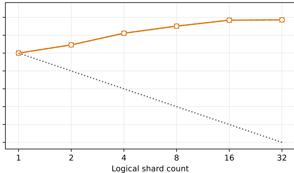
K-Means
