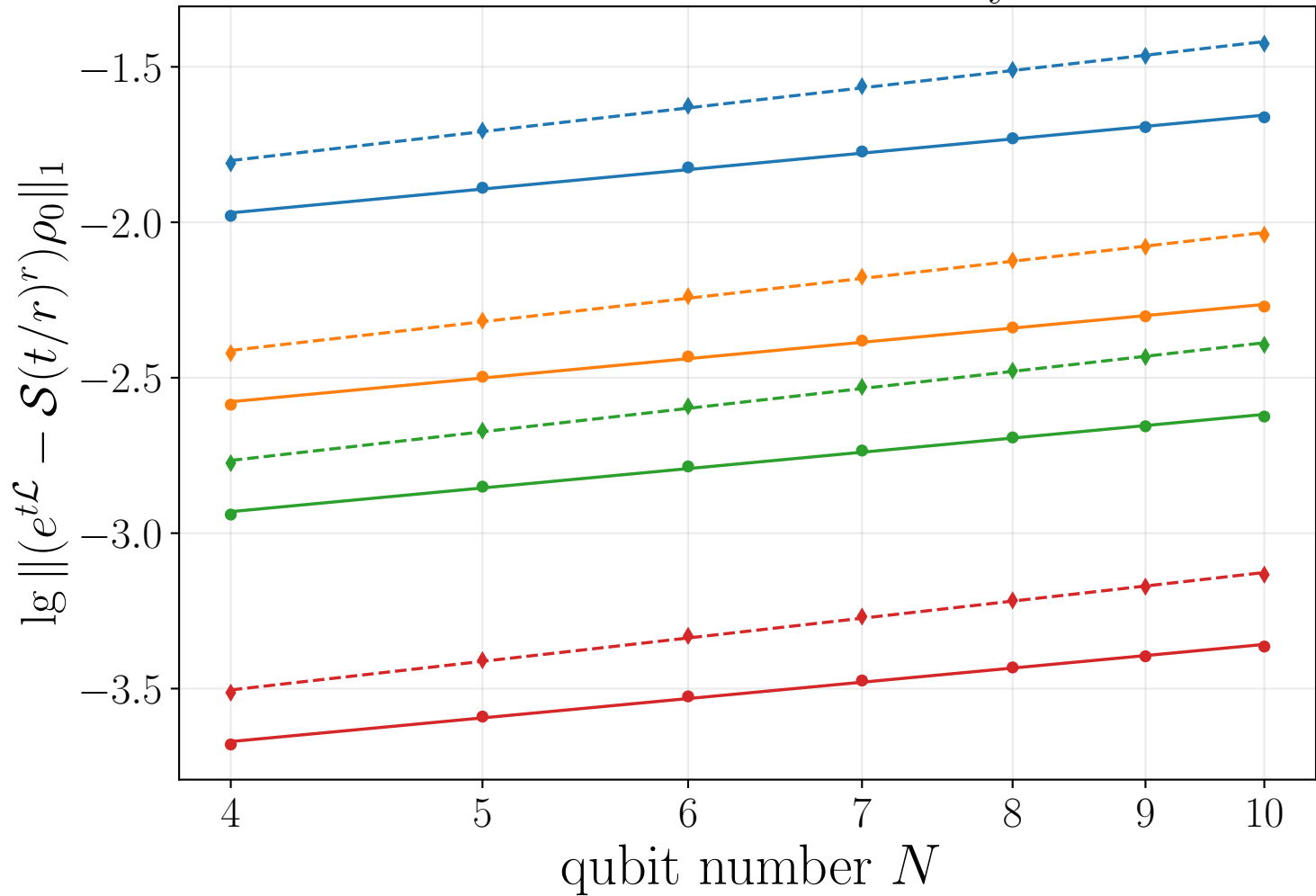
Lindbladian simulation error vs. system size N
