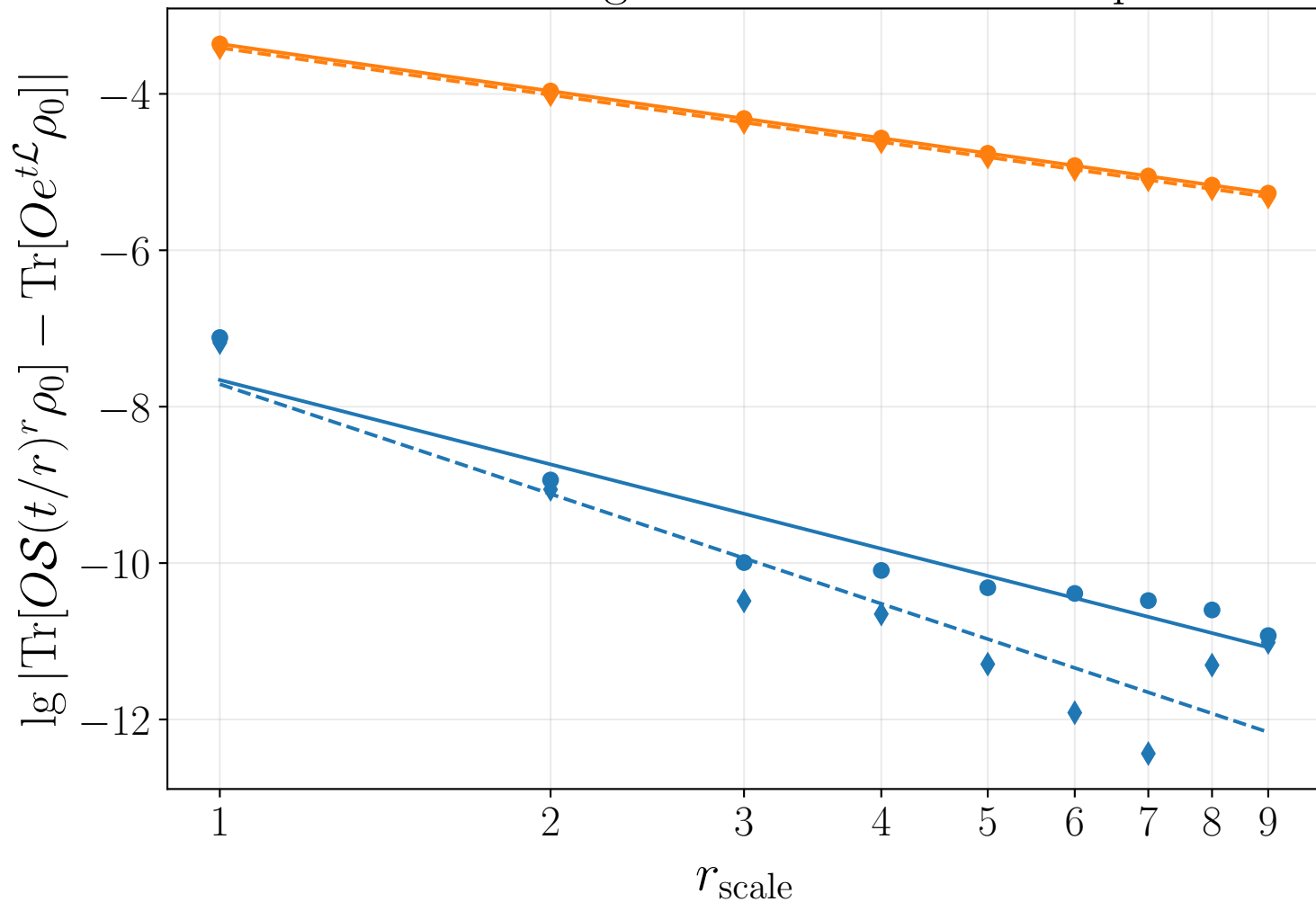
Trotter error scaling with Richardson extrapolation
