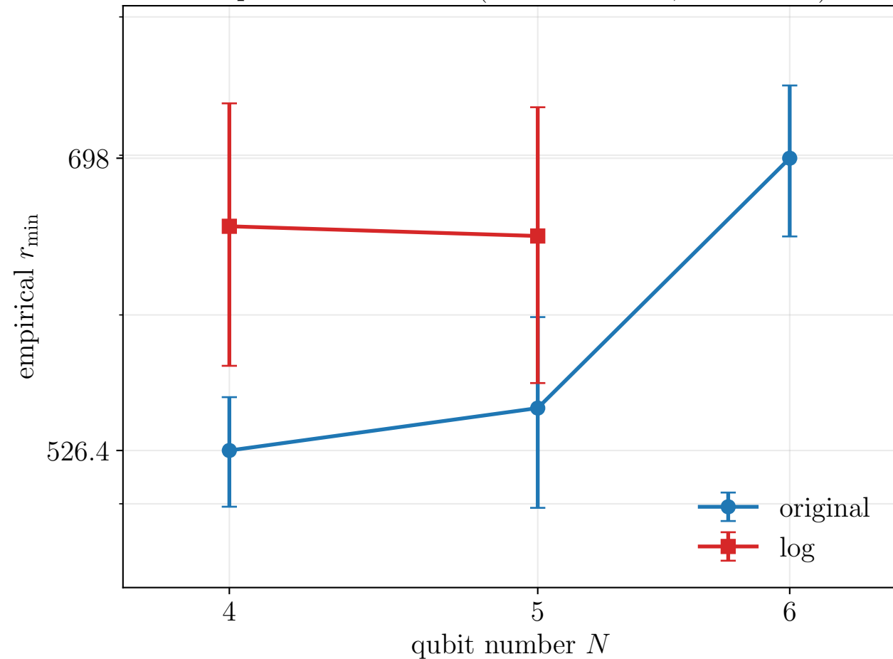
Empirical r_{\min} vs N (fixed T = 2.0 , \epsilon = 0.001 )
