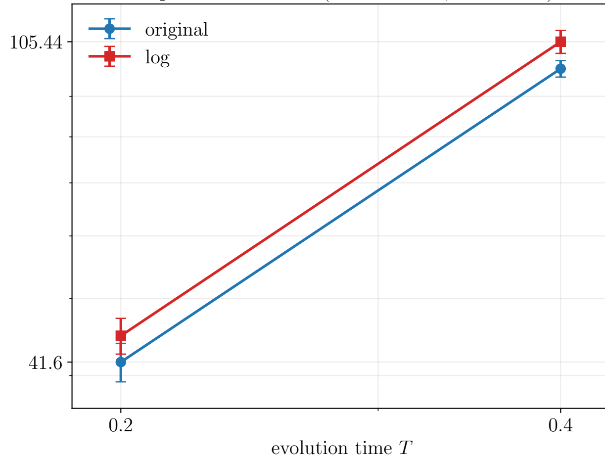
Empirical r_{\min} vs T (fixed N = 8 , \epsilon = 0.001 )
