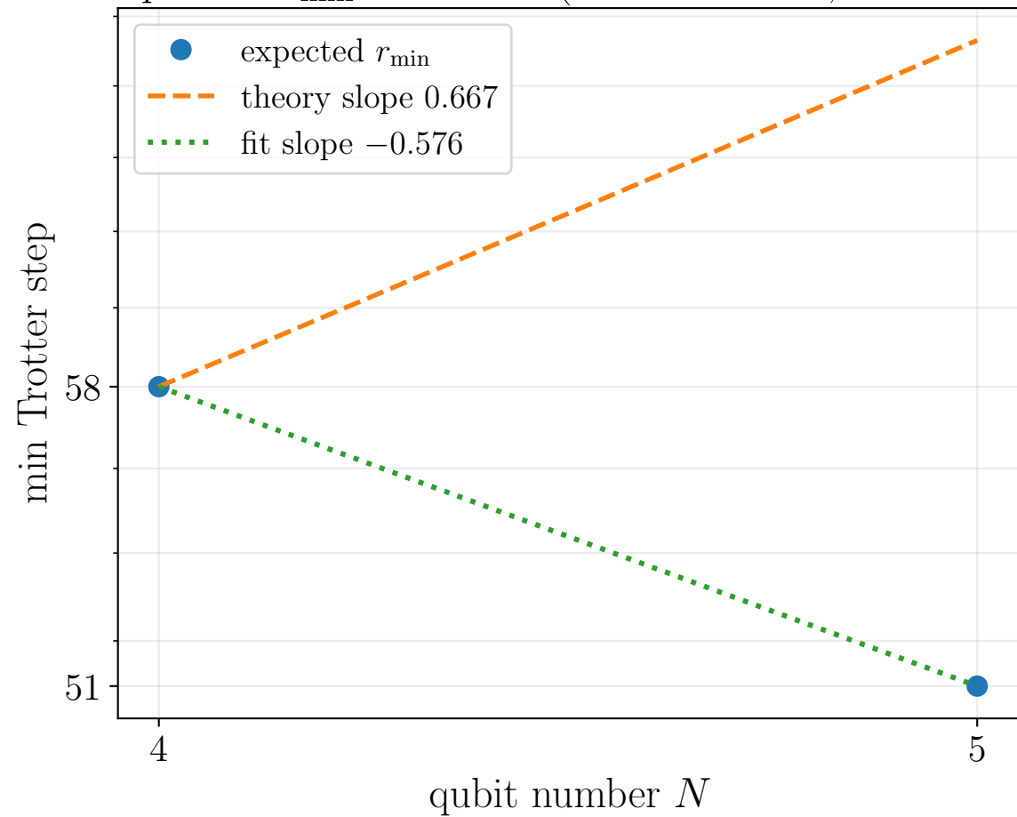
Expected r_{\min} versus N (fixed T = 2.0 , \epsilon = 0.001 )
