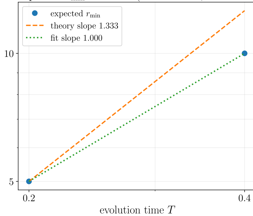
Expected r_{\min} versus T (fixed N = 8 , \epsilon = 0.001 )
