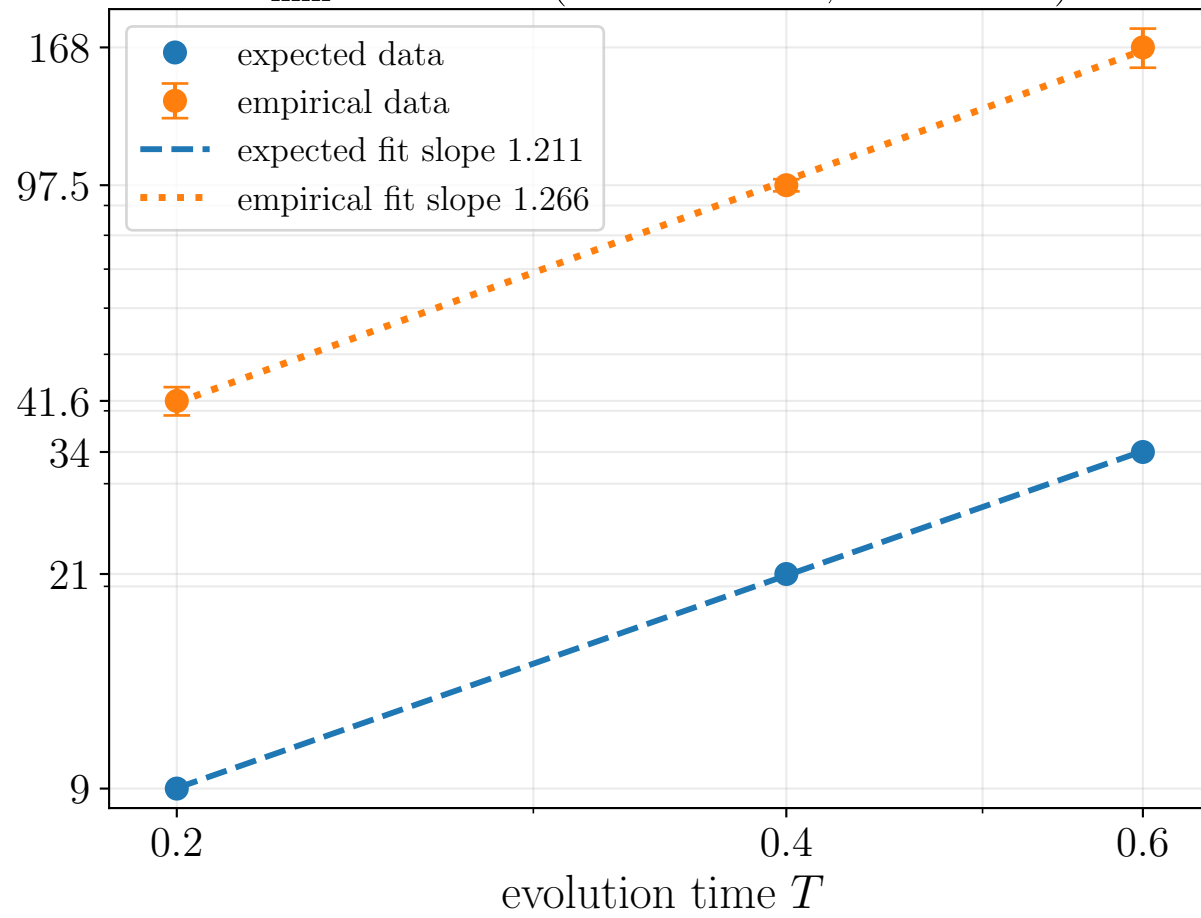
r_{\min} versus T (fixed N = 8 , \epsilon = 0.001 )
