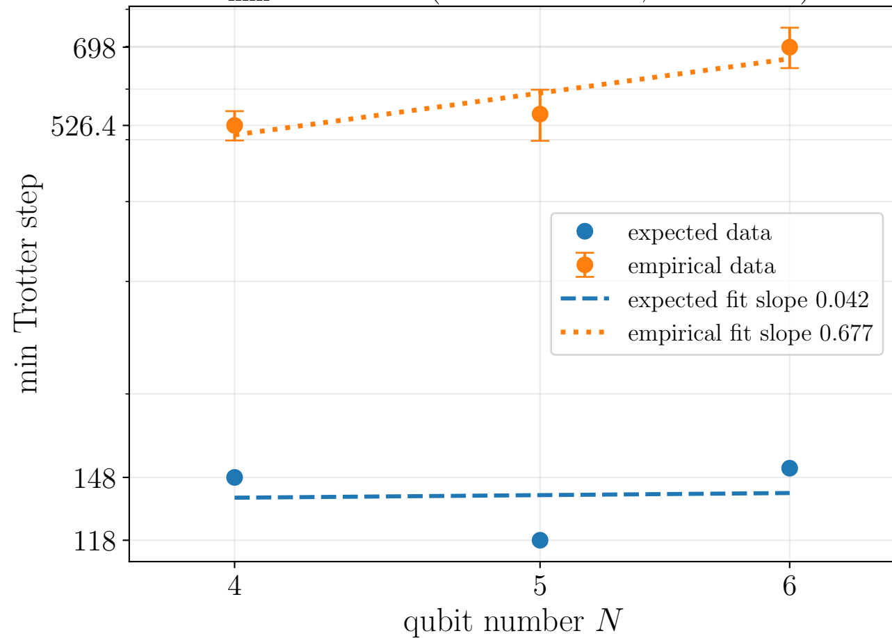
r_{\min} versus N (fixed T = 2.0 , \epsilon = 0.001 )
