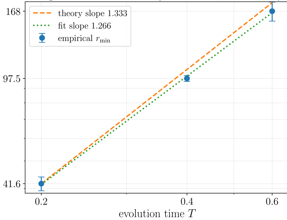
Empirical r_{\min} versus T (fixed N = 8 , \epsilon = 0.001 )
