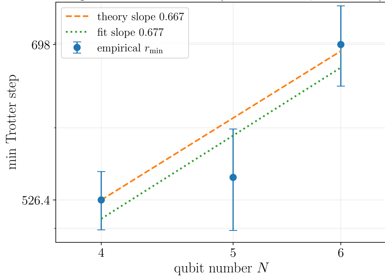
Empirical r_{\min} versus N (fixed T = 2.0 , \epsilon = 0.001 )
