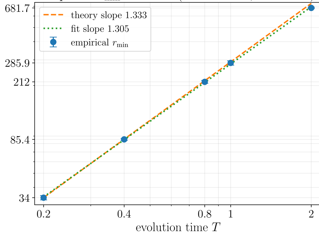
Empirical r_{\min} versus T (fixed N = 8 , \epsilon = 0.001 )
