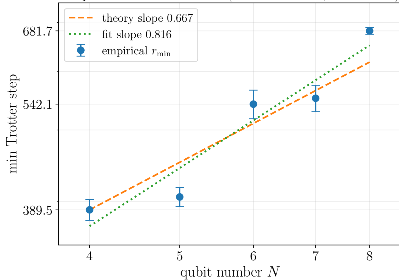
Empirical r_{\min} versus N (fixed T = 2.0 , \epsilon = 0.001 )
