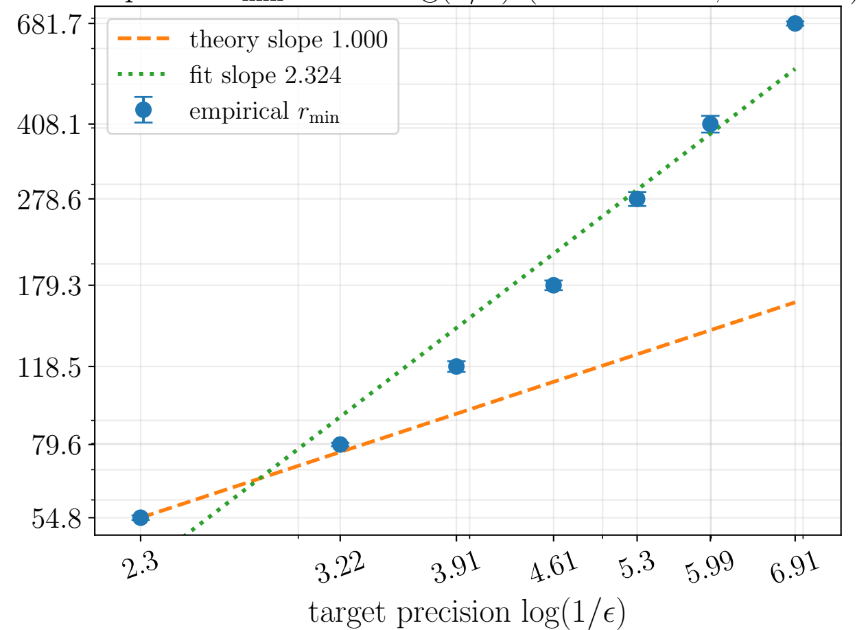
Empirical r_{\min} versus \log(1/\epsilon) (fixed N = 8 , T = 2.0 )
