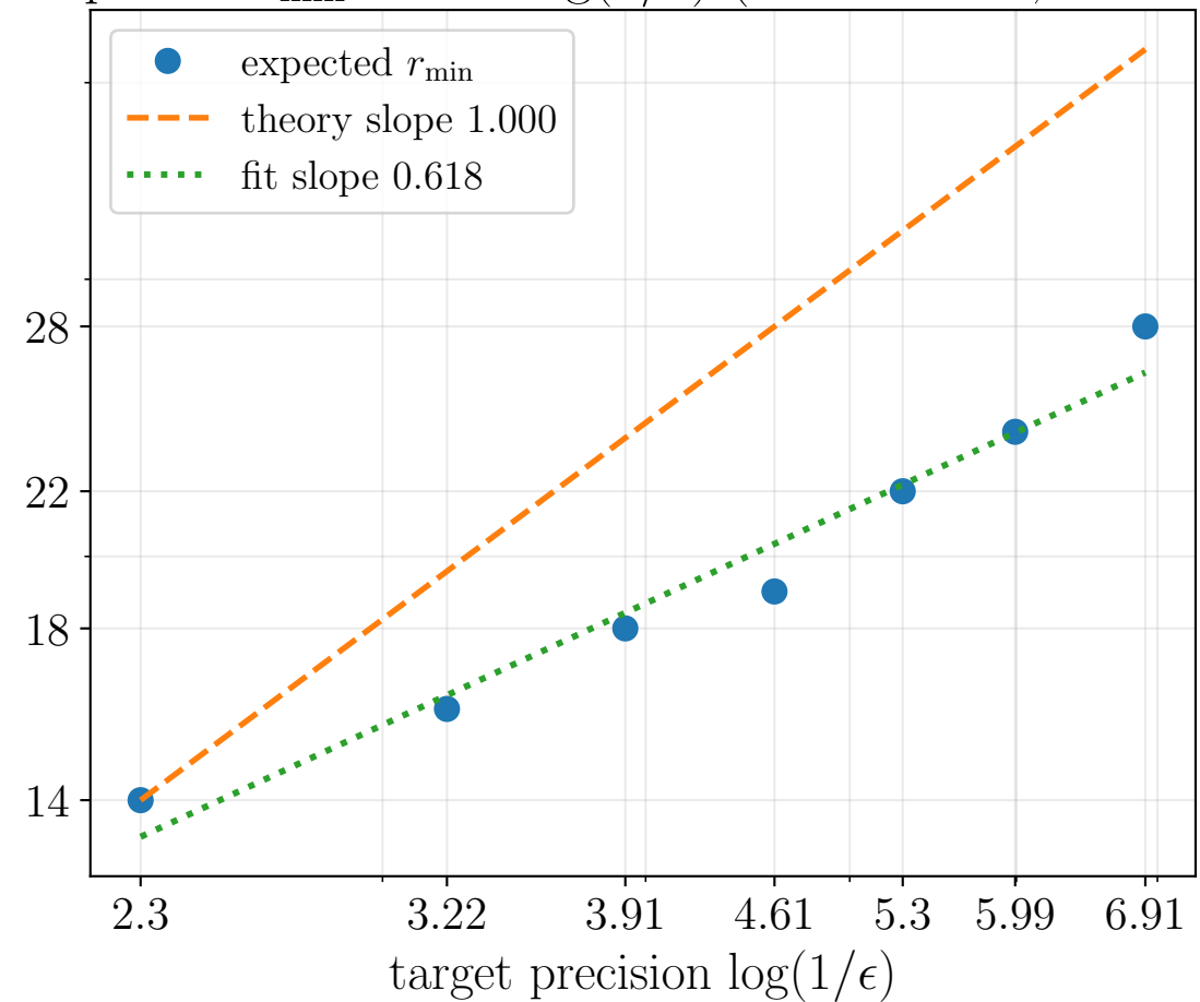
Expected r_{\min} versus \log(1/\epsilon) (fixed N = 8 , T = 2.0 )
