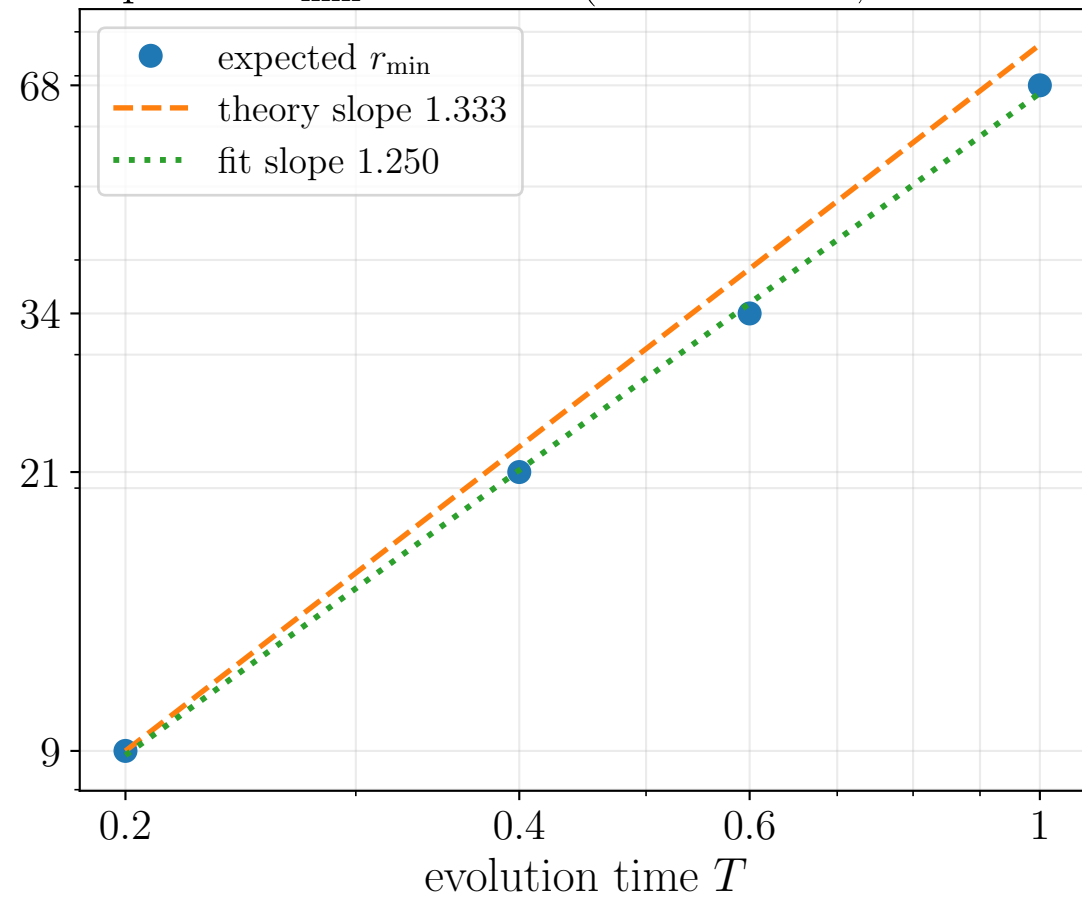
Expected r_{\min} versus T (fixed N = 8 , \epsilon = 0.001 )
