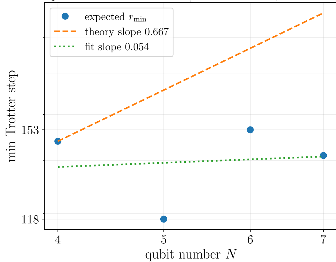
Expected r_{\min} versus N (fixed T = 2.0 , \epsilon = 0.001 )
