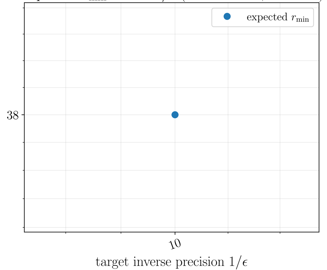
Expected r_{\min} versus 1/\epsilon (fixed N = 8 , T = 2.0 )
