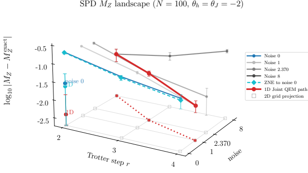
FIG. 4. Richardson extrapolation landscape obtained from sparse Pauli dynamics for the simulated 100-qubit open Ising chain. The observable is the average longitudinal magnetization M_Z = N^{-1} \sum_i Z_i , and the error is plotted as \log_{10} |M_Z - M_Z^{\text{exact}}| . The Hamiltonian convention follows Eq. (6); using R_P(\theta) = e^{-i\theta P/2} , the parameters are \theta_h = \theta_J = -2 . The one-dimensional path uses the inverse-cubic paired nodes (r, \lambda) \in \{(2, 8), (3, 64/27), (4, 1)\} , while the two-dimensional comparison uses the rectangular grid r \in \{2, 3, 4\} and \lambda \in \{0, 1, 64/27, 8\} . The reference value M_Z^{\text{exact}} denotes the corresponding exact noiseless expectation. Error bars are obtained by propagating the trajectory-level standard errors in the observable M_Z before mapping the resulting intervals to the logarithmic error axis. Fixed-noise slices show the noisy data across Trotter step counts, cyan diamonds show zero-noise extrapolations at fixed r , and the red curve marks the one-dimensional joint-QEM path. Open squares indicate the projection of the corresponding two-dimensional Richardson construction.
