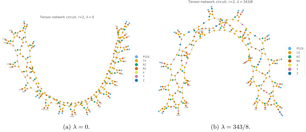
Figure S5: Tensor-network graph representations of representative product-formula circuits, retained here as circuit-structure illustrations. Both panels use the local illustrative setup N = 20 , J = h = T = 1 , r = 2 and a fixed random seed. The noisy panel corresponds to \lambda = 343/8 in this illustrative setup. The displayed graphs are generated by quimb ; SVG vector versions are provided with the source files.
