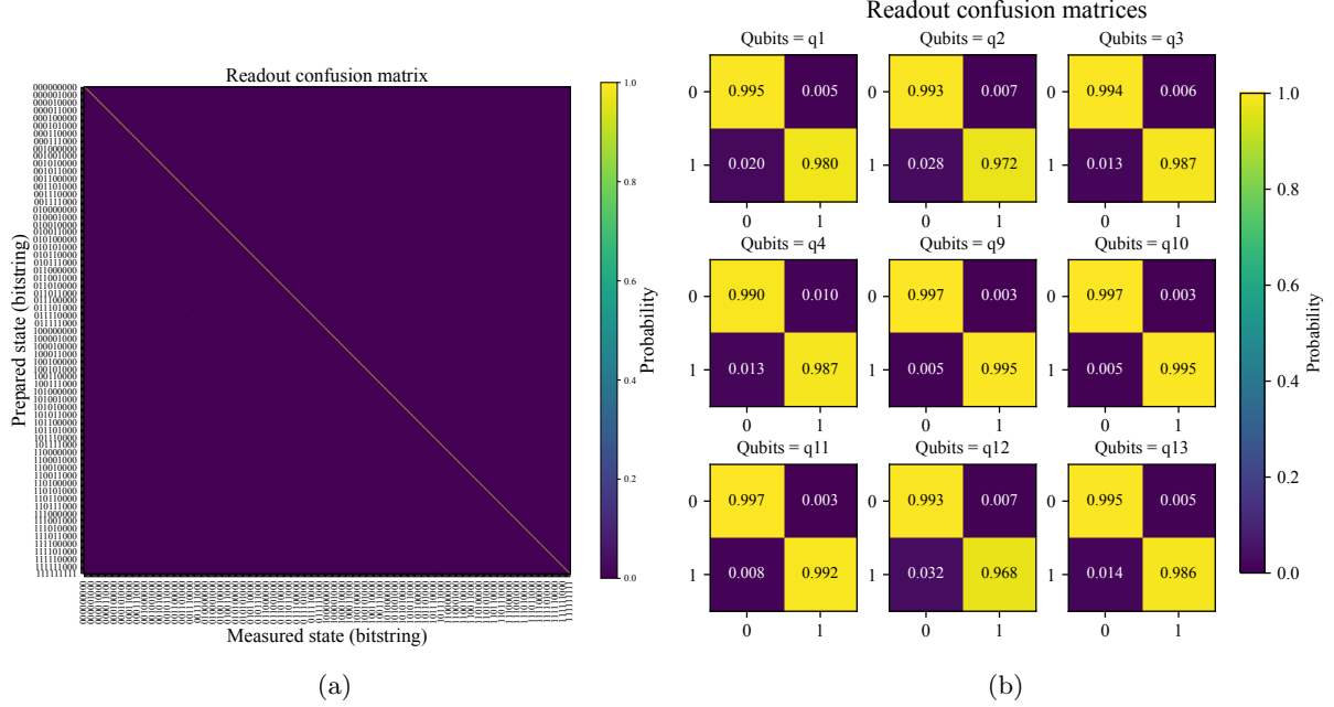
Figure S2: Data to be aligned Readout calibration data for the selected 9-qubit device subgraph. (a) Full 2^9 \times 2^9 global confusion matrix, whose entries give the conditional probabilities of measured bitstrings given prepared computational-basis states. (b) Single-qubit local calibration matrices used for observable-level readout mitigation of the magnetization. The diagonal dominance of the calibration data supports local observable-level correction for the measured average magnetization.
