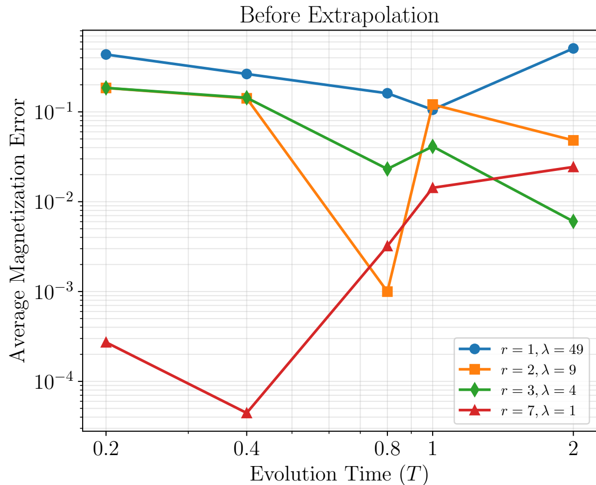
Error vs Evolution Time ( N = 20 )
