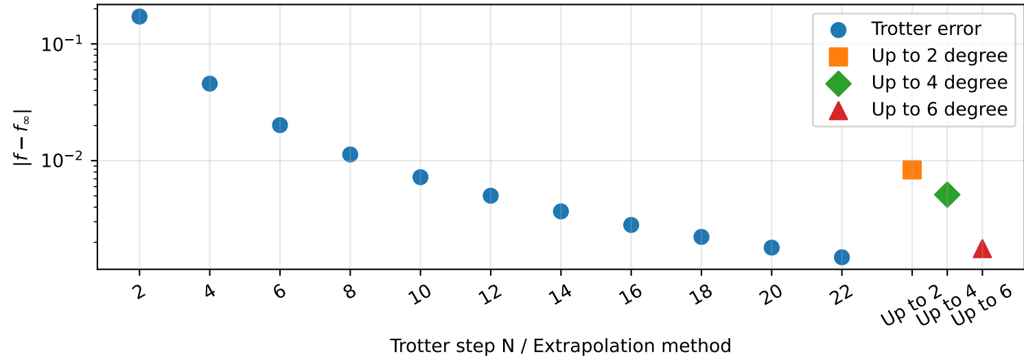
Trotter Error and Hardware Extrapolation Errors
