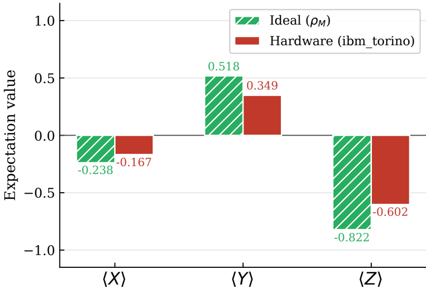
(b) Pauli expectation values
